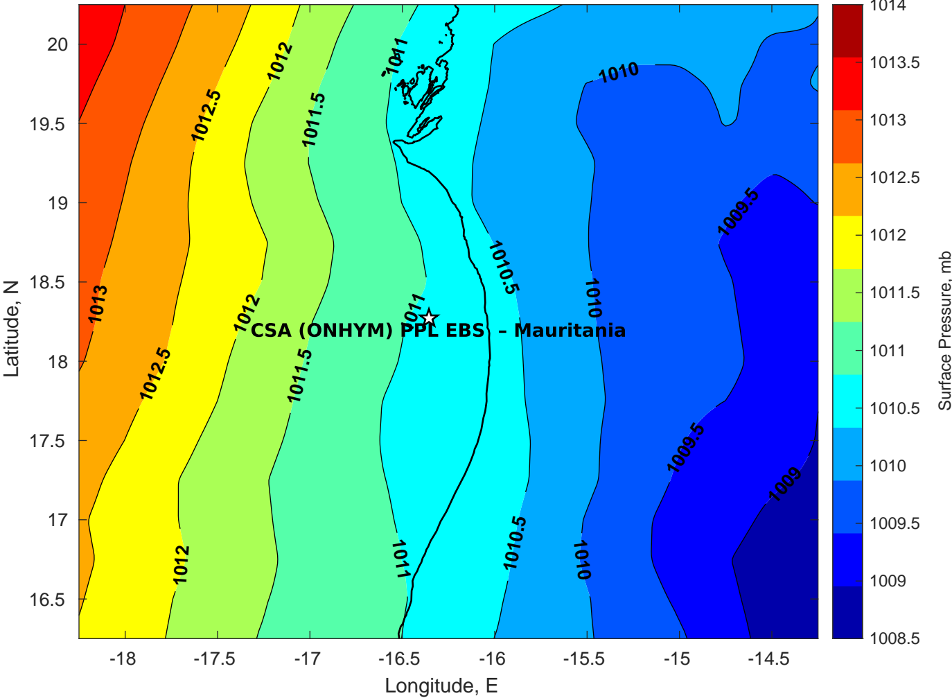
Surface Pressure (mb) for CSA (ONHYM) PPL EBS - Mauritania at 13-Feb-2025 00:00:00
