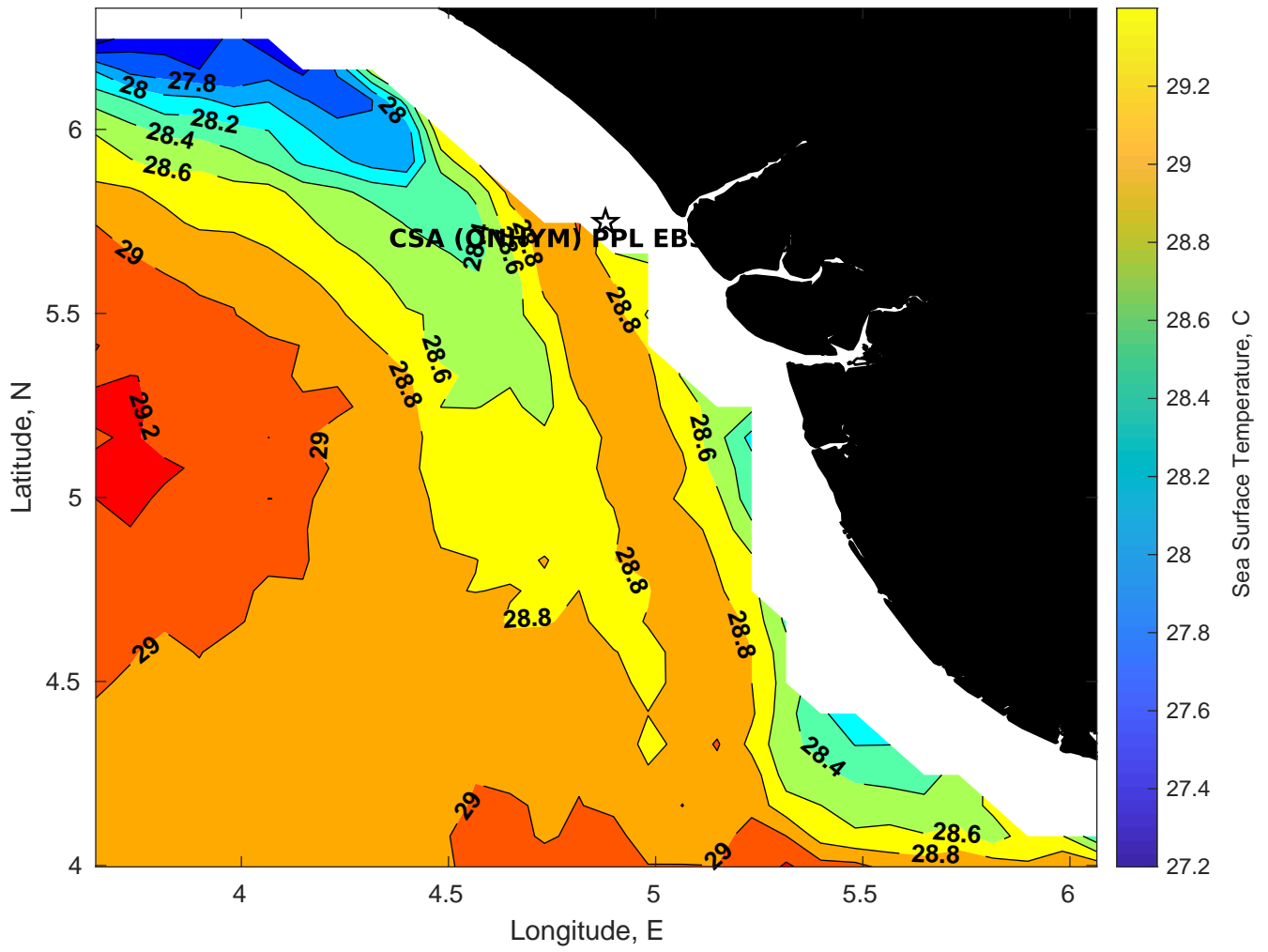
SST for CSA (ONHYM) PPL EBS - Nigeria at 11-Feb-2025 00:00:00
