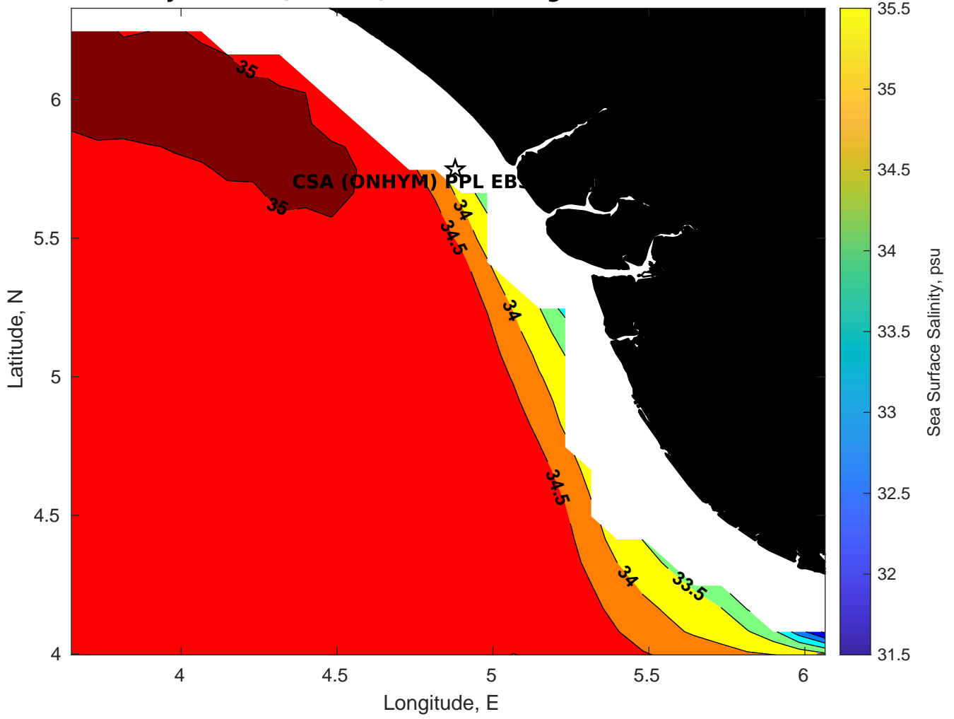
Surface Salinity for CSA (ONHYM) PPL EBS - Nigeria at 11-Feb-2025 00:00:00
