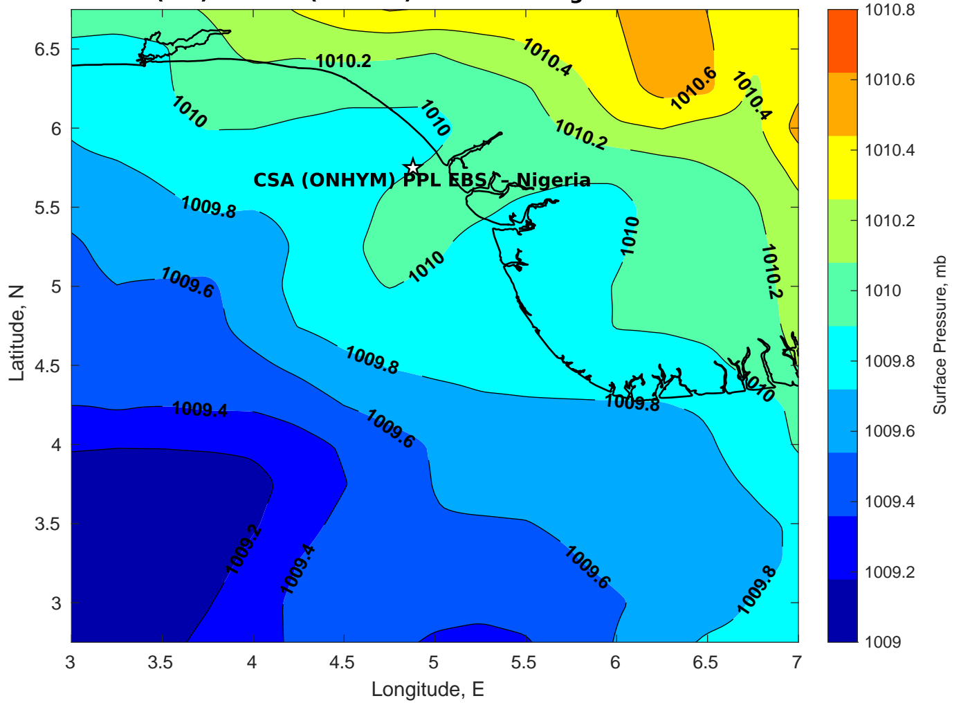
Surface Pressure (mb) for CSA (ONHYM) PPL EBS - Nigeria at 14-Feb-2025 06:00:00
