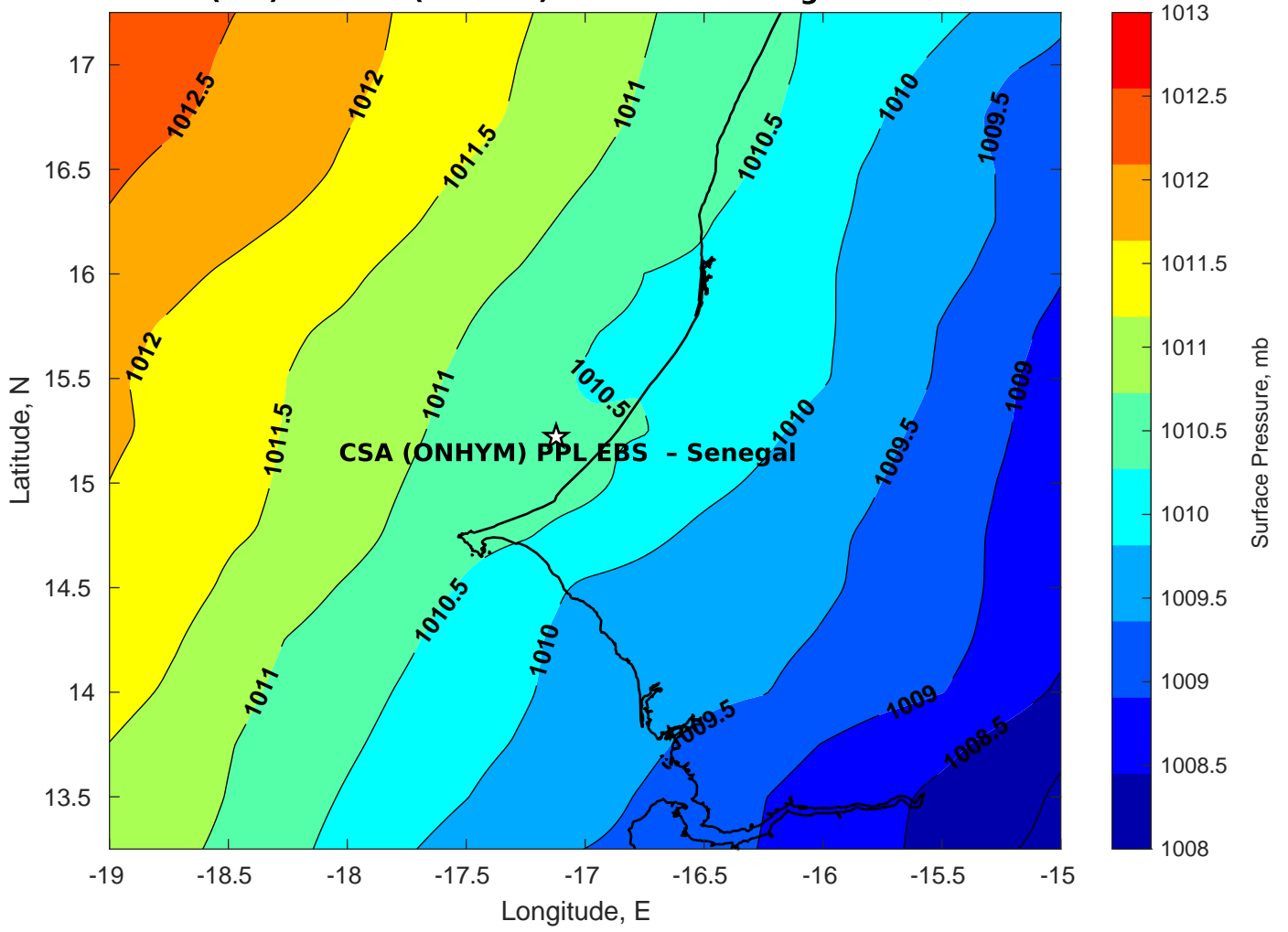
Surface Pressure (mb) for CSA (ONHYM) PPL EBS - Senegal at 12-Feb-2025 00:00:00
