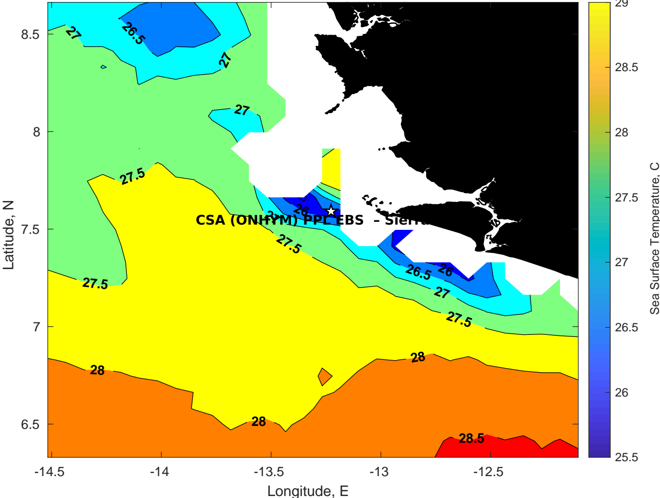
SST for CSA (ONHYM) PPL EBS - Sierra Leone at 11-Feb-2025 00:00:00
