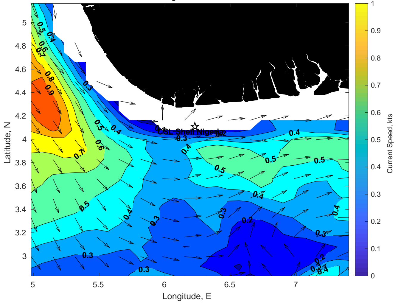
Surface Currents for CSL Shell Nigeria at 11-Feb-2025 00:00:00
