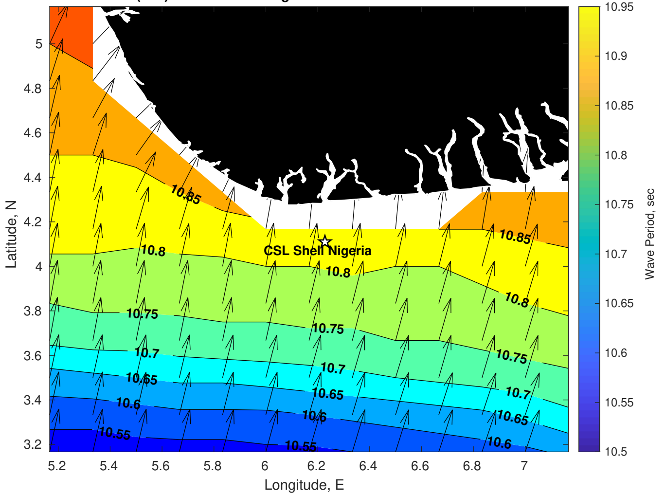
Wave Period (sec) for CSL Shell Nigeria at 12-Feb-2025 09:00:00
