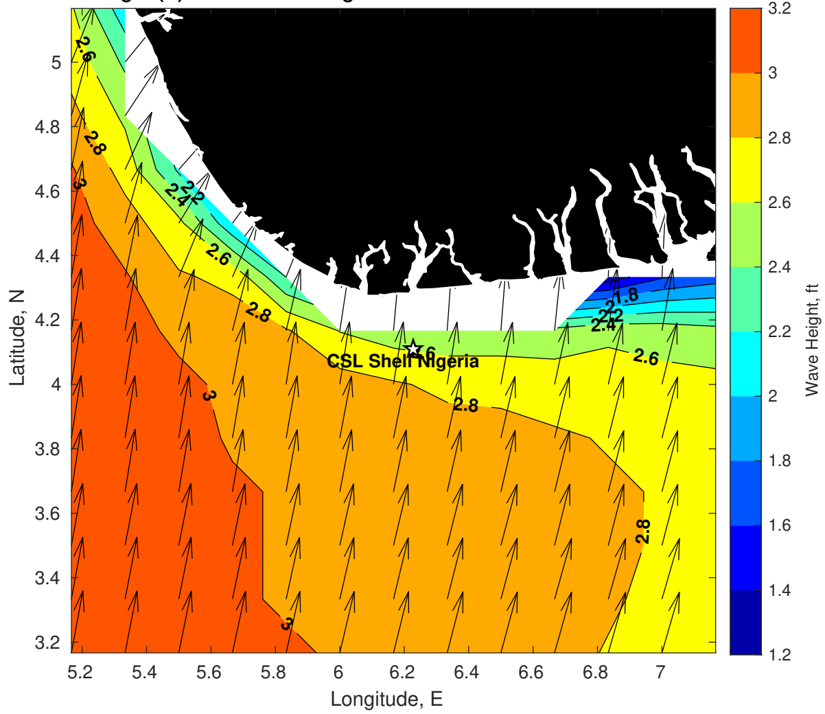
Wave Height (ft) for CSL Shell Nigeria at 12-Feb-2025 09:00:00
