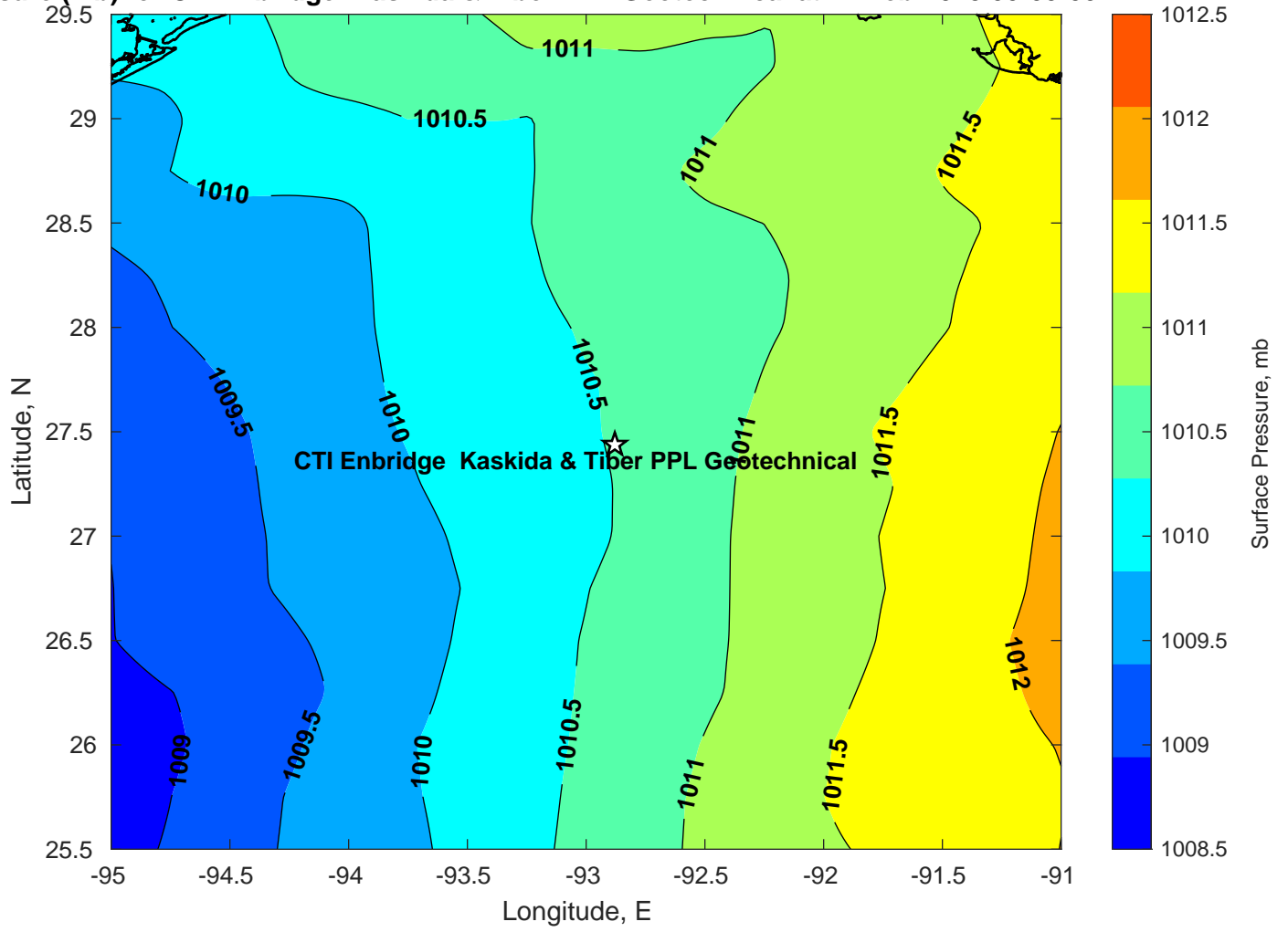
Surface Pressure (mb) for CTI Enbridge Kaskida & Tiber PPL Geotechnical at 12-Feb-2025 00:00:00
