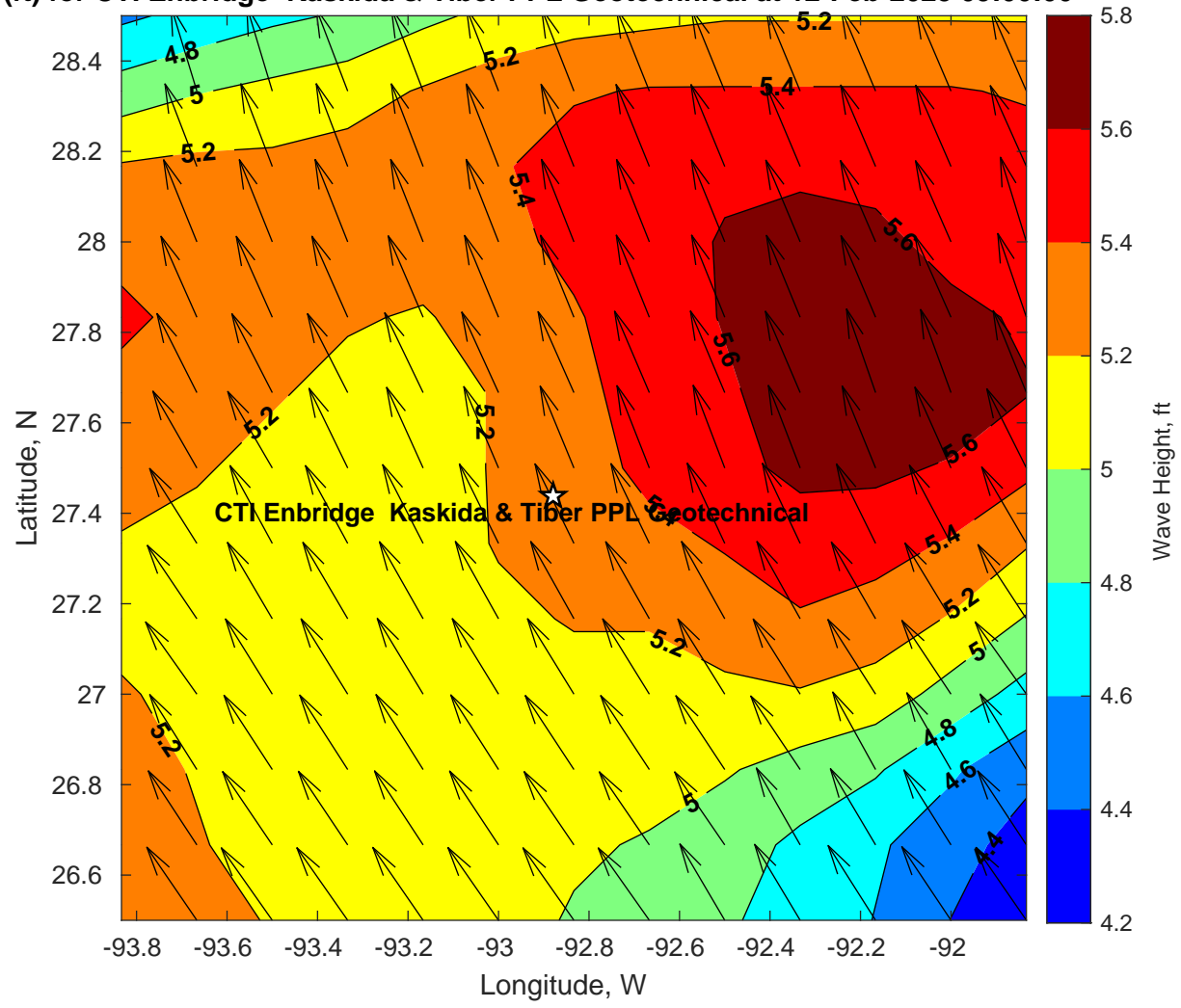
Wave Height (ft) for CTI Enbridge Kaskida & Tiber PPL Geotechnical at 12-Feb-2025 09:00:00
