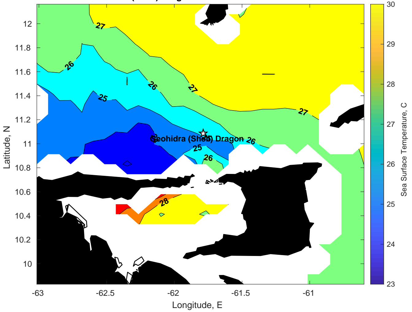
SST for Geohdra (Shell) Dragon at 11-Feb-2025 00:00:00
