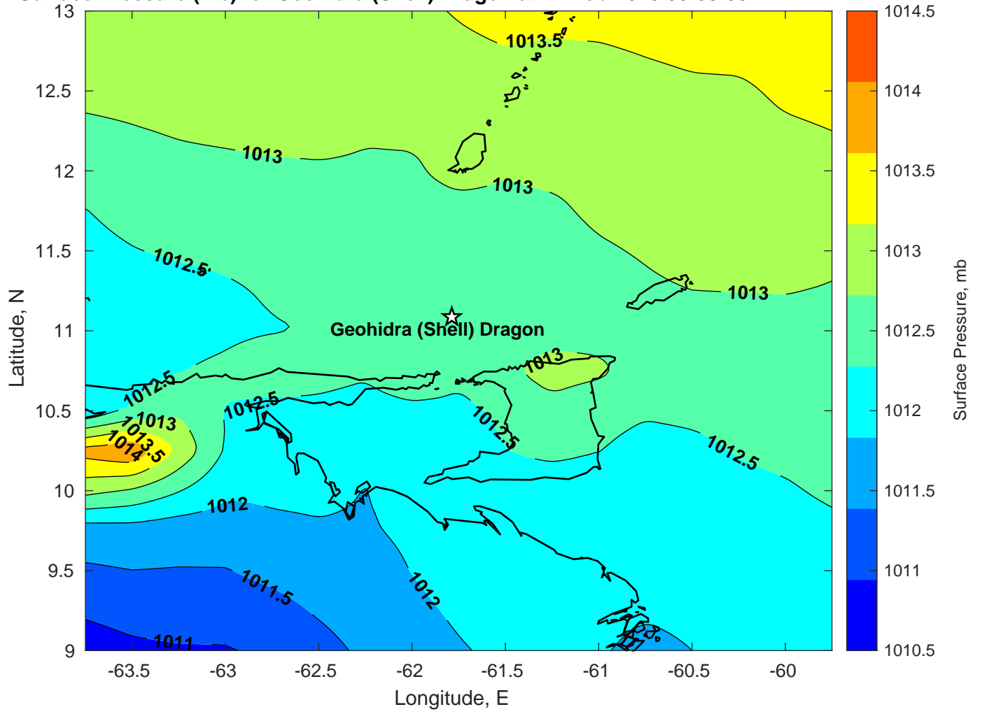
Surface Pressure (mb) for Geohidra (Shell) Dragon at 12-Feb-2025 00:00:00
