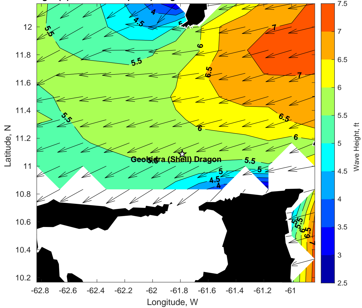
Wave Height (ft) for Geohidra (Shell) Dragon at 12-Feb-2025 09:00:00
