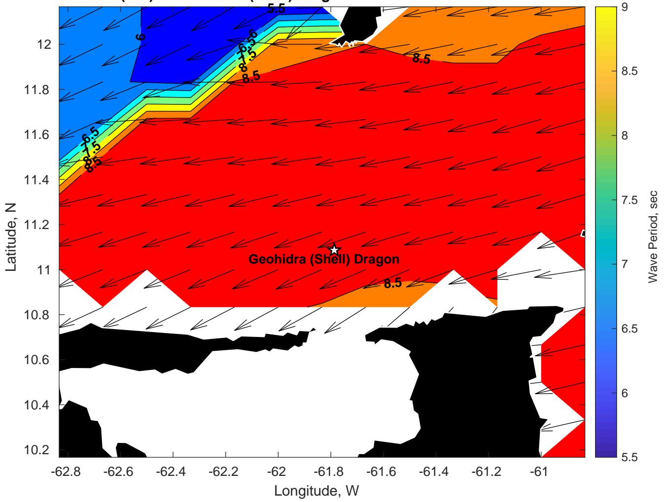
Wave Period (sec) for Geohidra (Shell) Dragon at 12-Feb-2025 09:00:00
