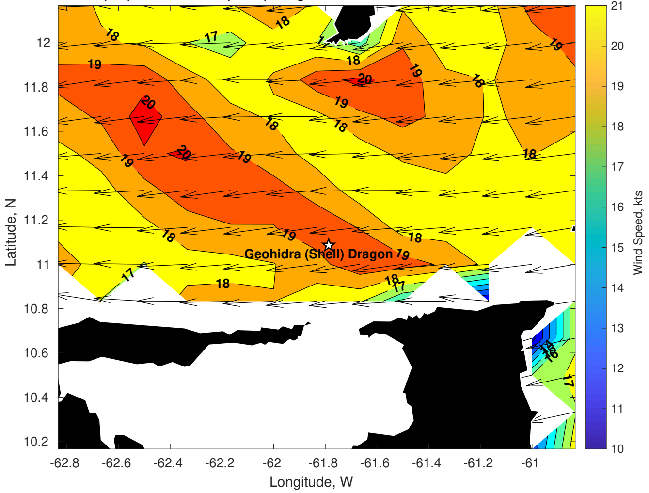
Winds (kts) for Geohidra (Shell) Dragon at 12-Feb-2025 09:00:00
