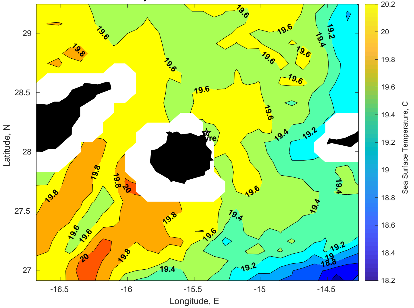
SST for Gyre at 11-Feb-2025 00:00:00
