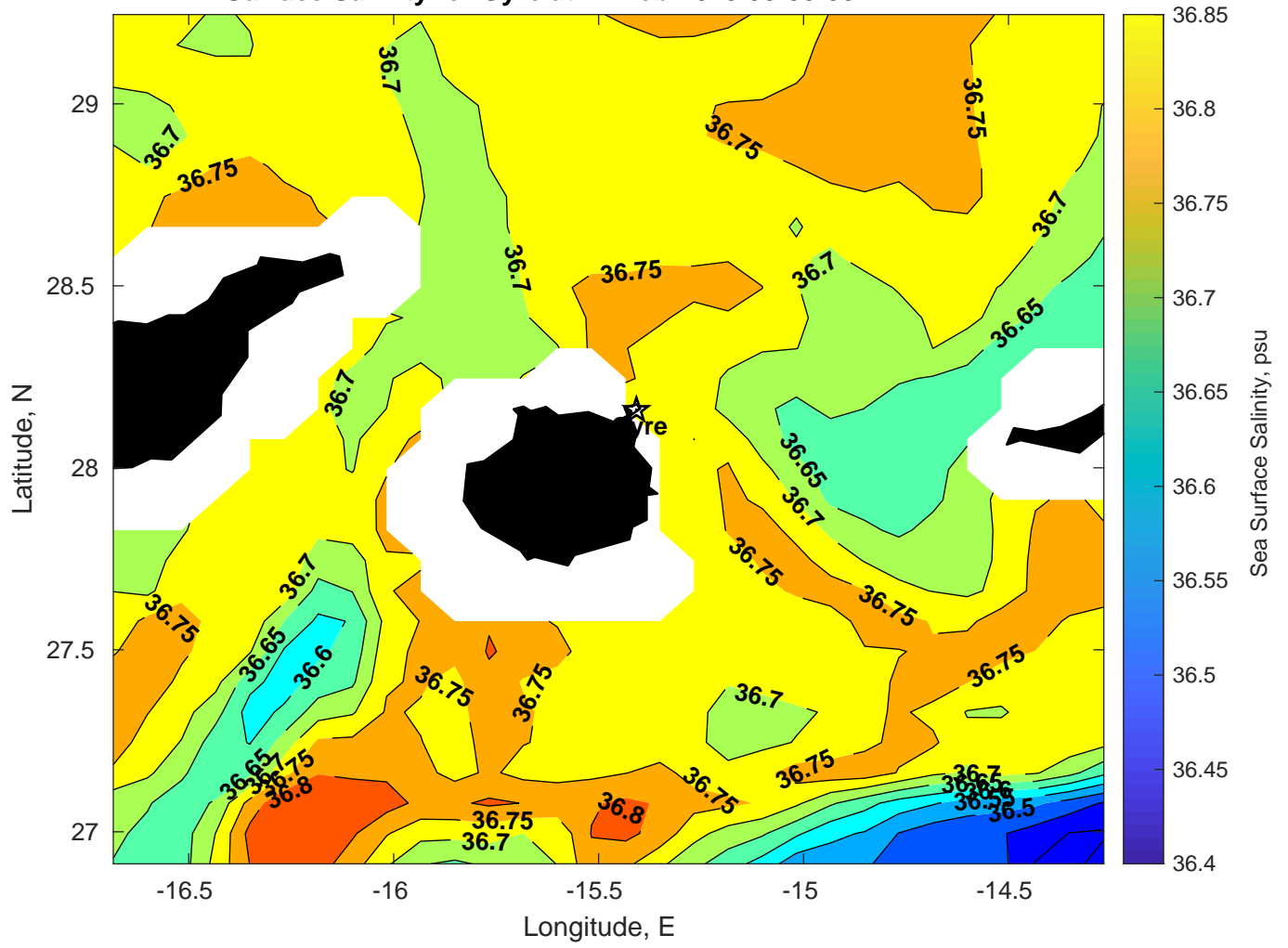
Surface Salinity for Gyre at 11-Feb-2025 00:00:00
