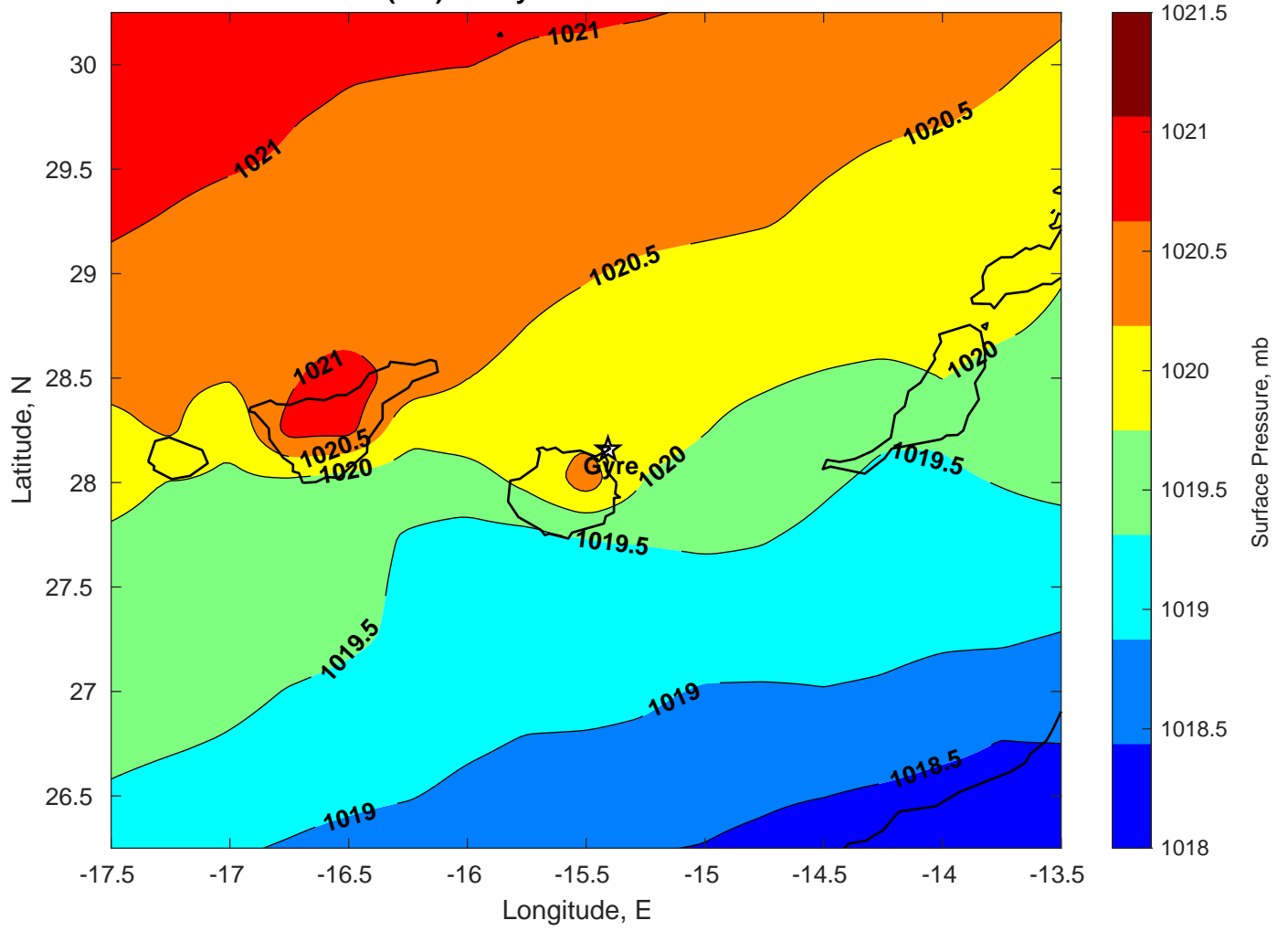
Surface Pressure (mb) for Gyre at 12-Feb-25 00:00:00
