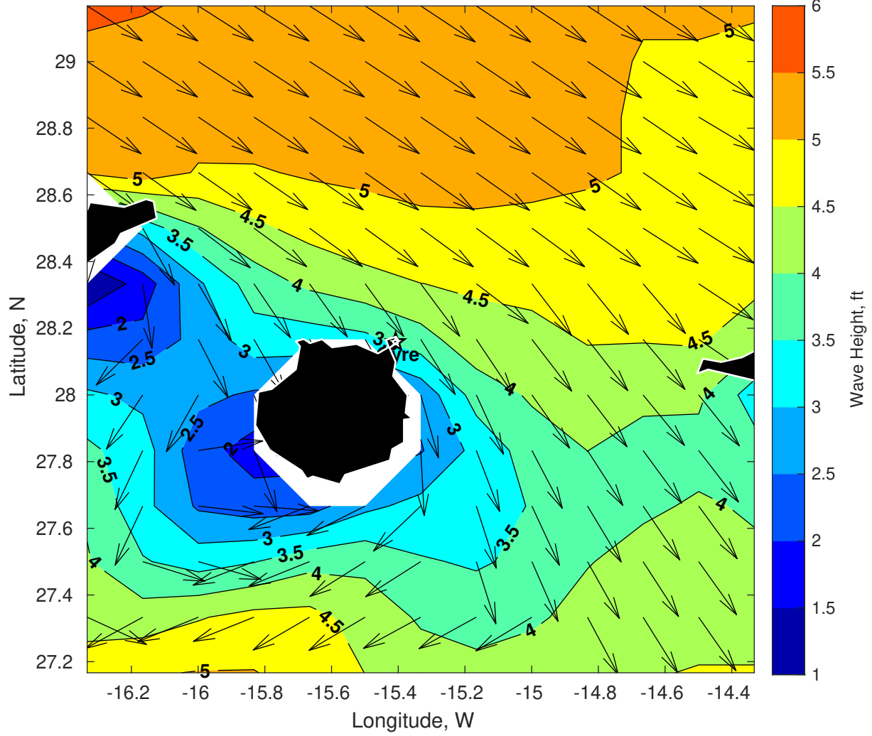
Wave Height (ft) for Gyre at 12-Feb-2025 09:00:00
