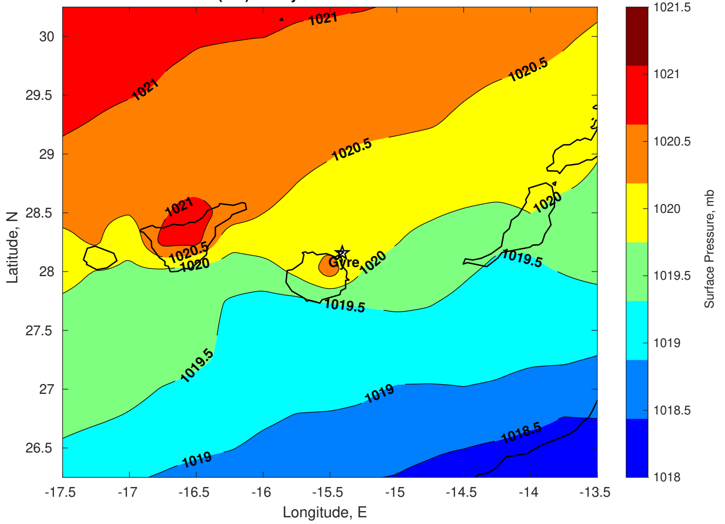
Surface Pressure (mb) for Gyre at 12-Feb-2025 00:00:00
