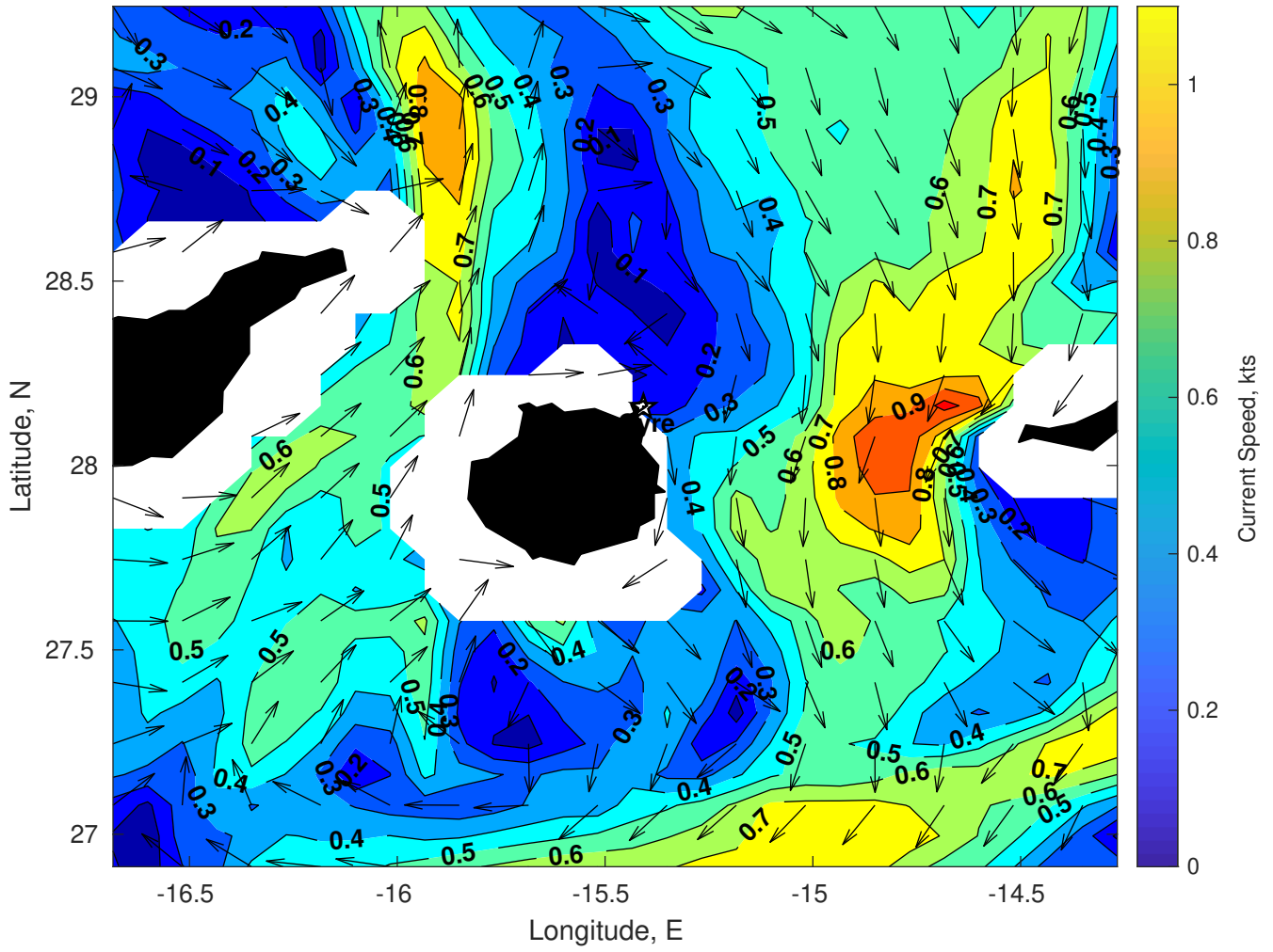
Surface Currents for Gyre at 11-Feb-2025 00:00:00
