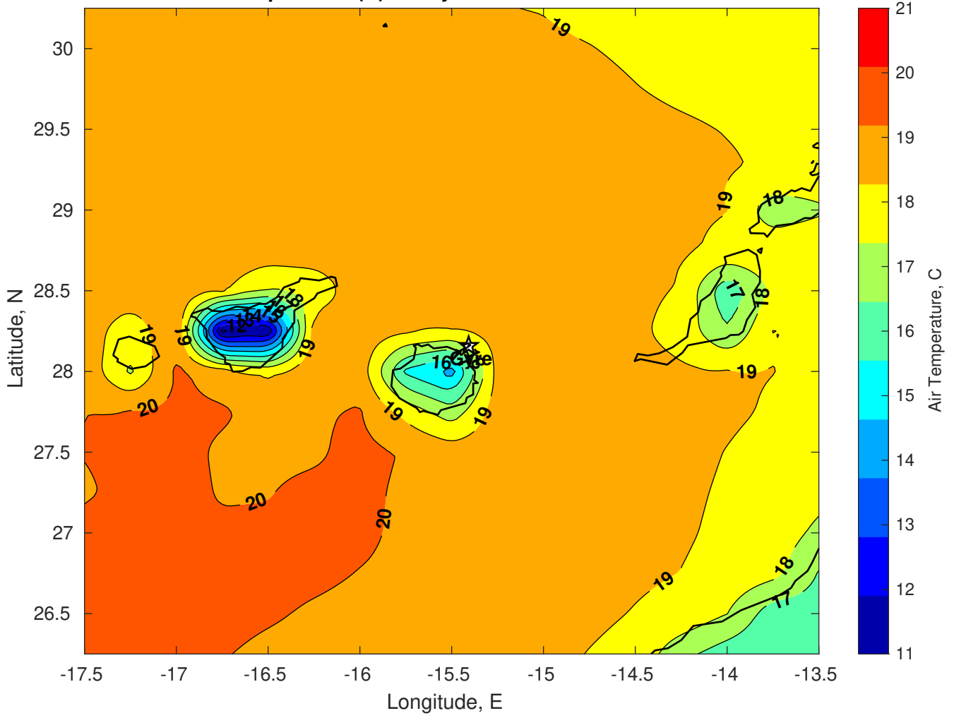
Air Temperature (C) for Gyre at 12-Feb-2025
