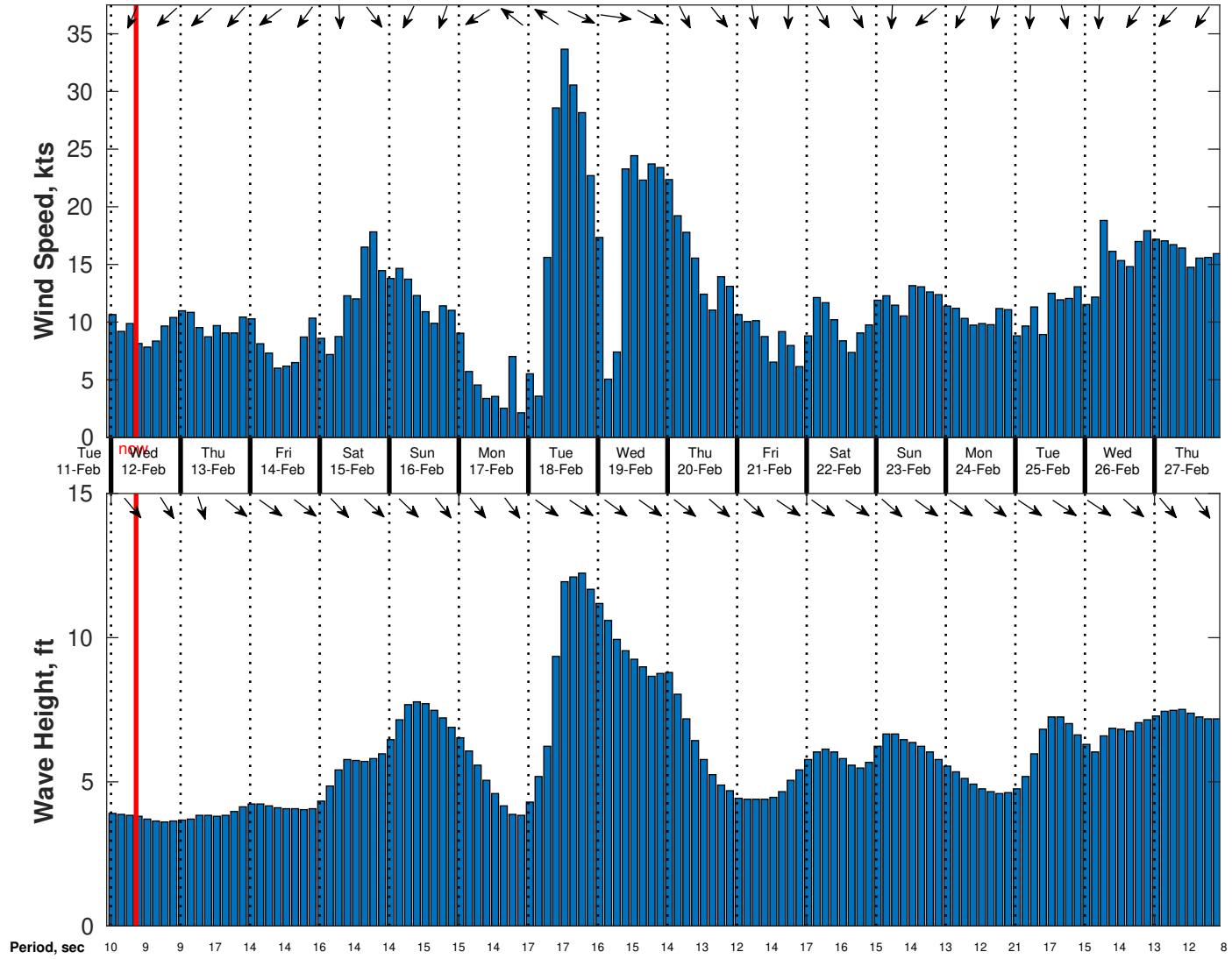
Wind & Wave Forecast for Gyre from 11-Feb-2025 23:00:00 to 27-Feb-2025 23:00:00
