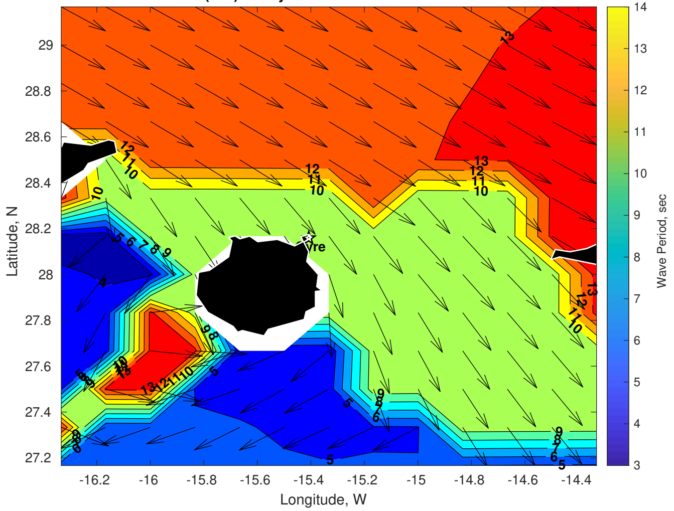
Wave Period (sec) for Gyre at 12-Feb-2025 09:00:00
