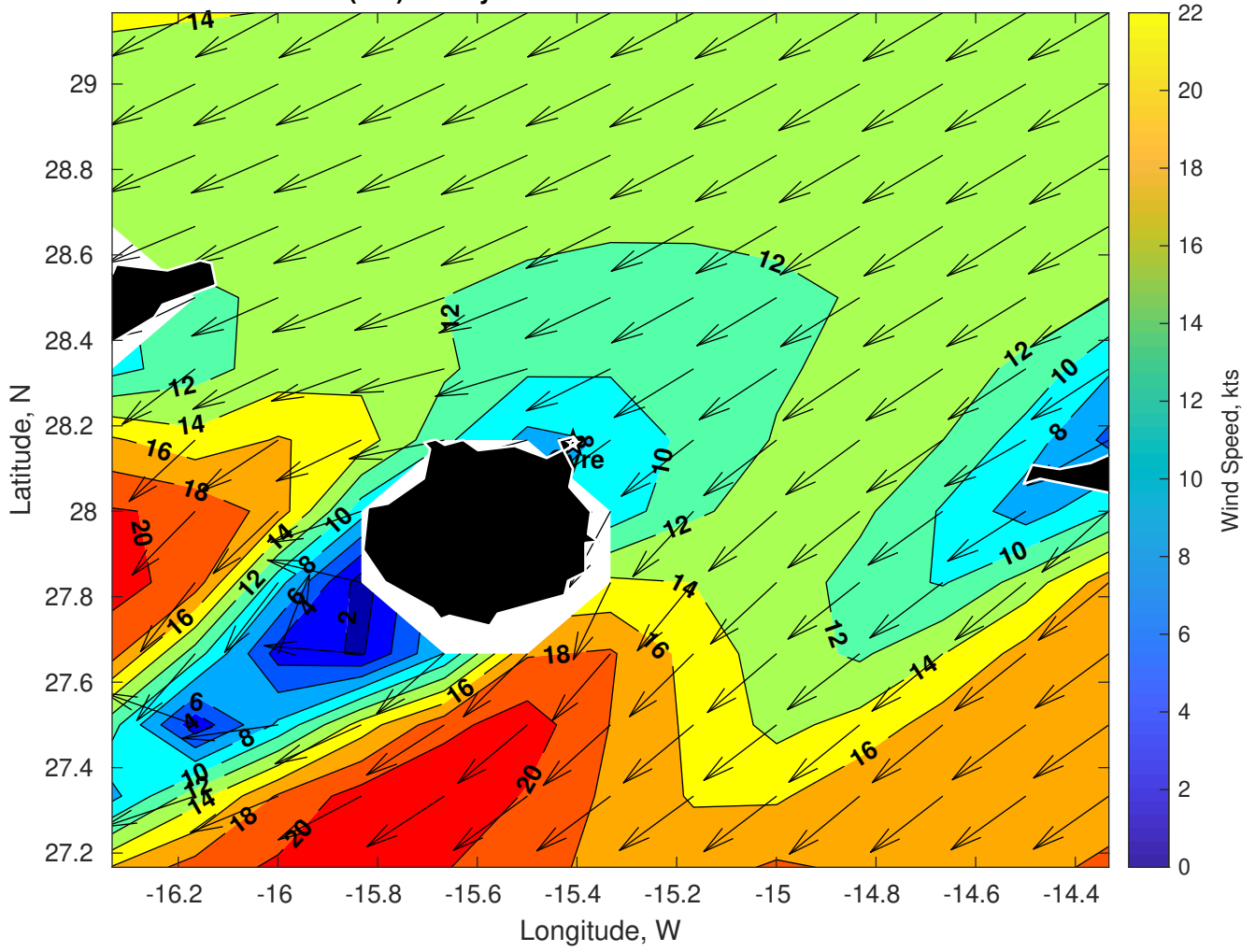
Winds (kts) for Gyre at 12-Feb-2025 09:00:00
