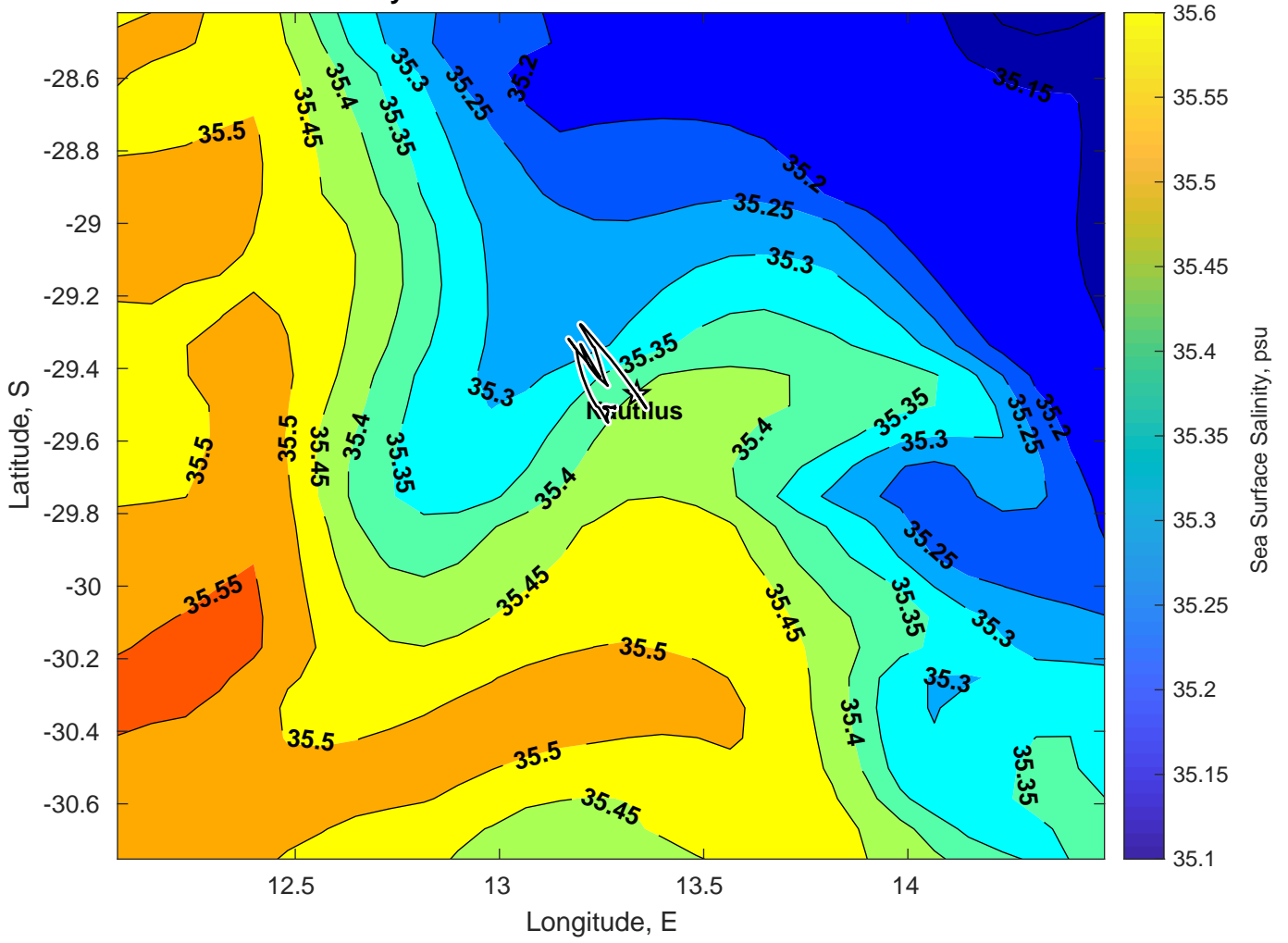
Surface Salinity for Nautilus at 11-Feb-2025 00:00:00
