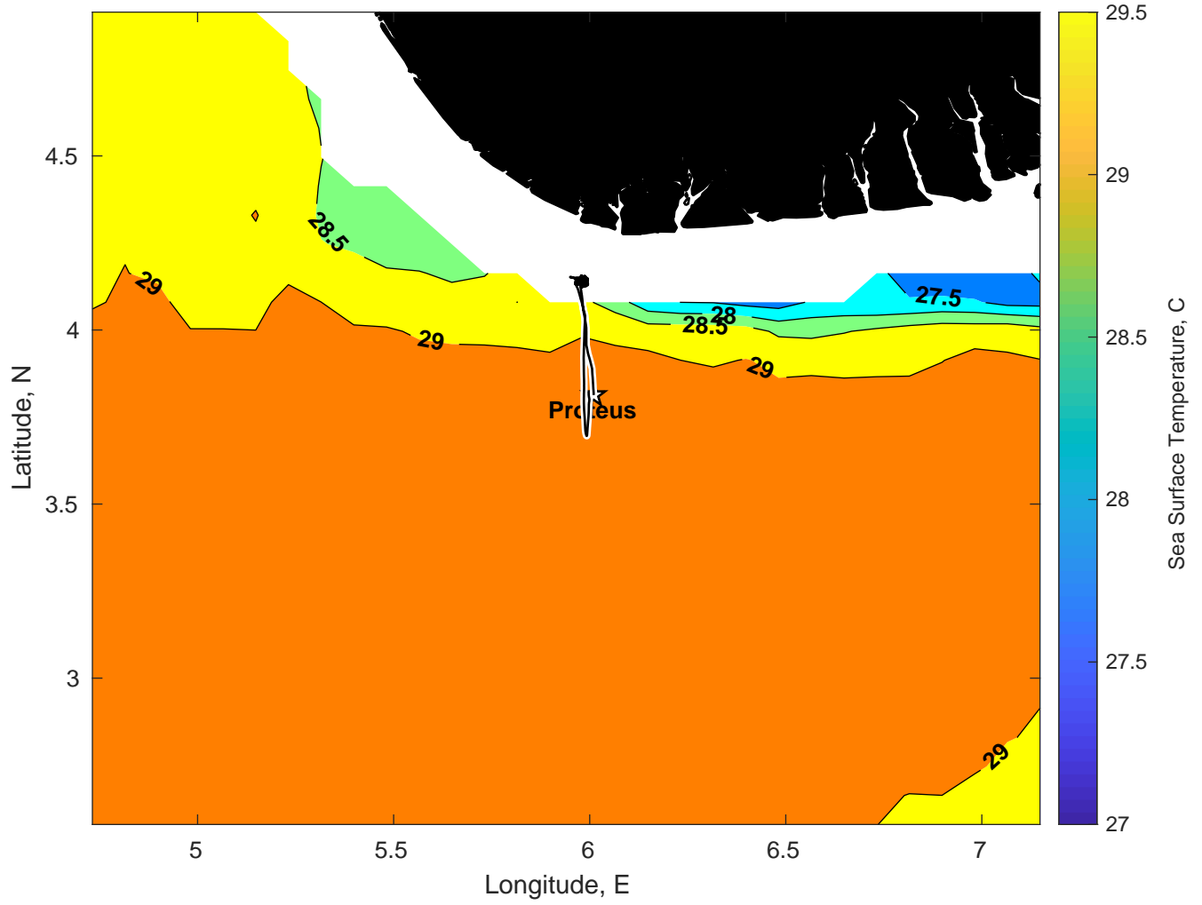
SST for Proteus at 11-Feb-2025 00:00:00
