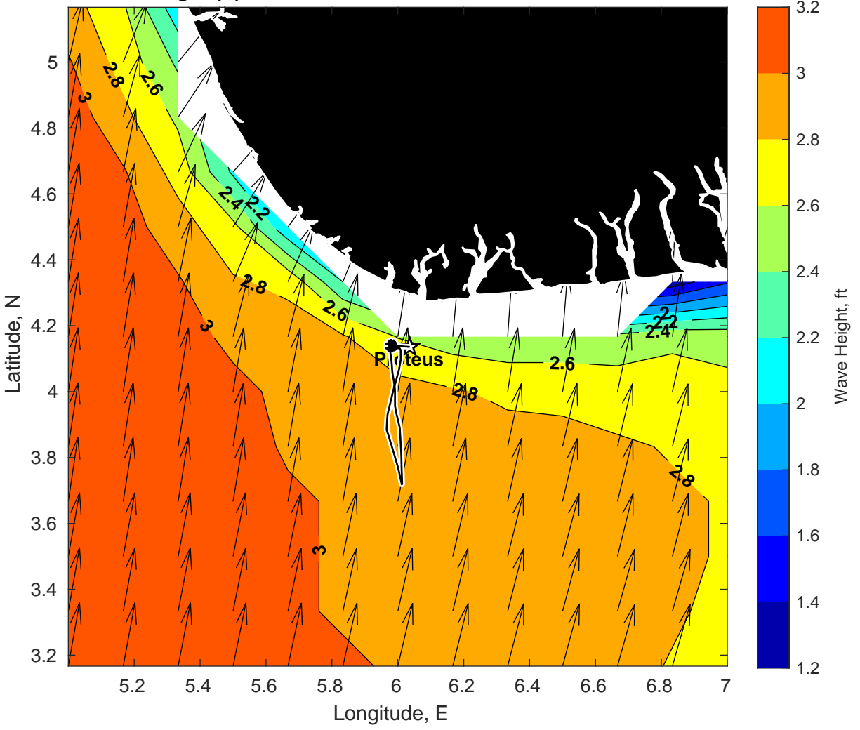
Wave Height (ft) for Proteus at 12-Feb-2025 09:00:00
