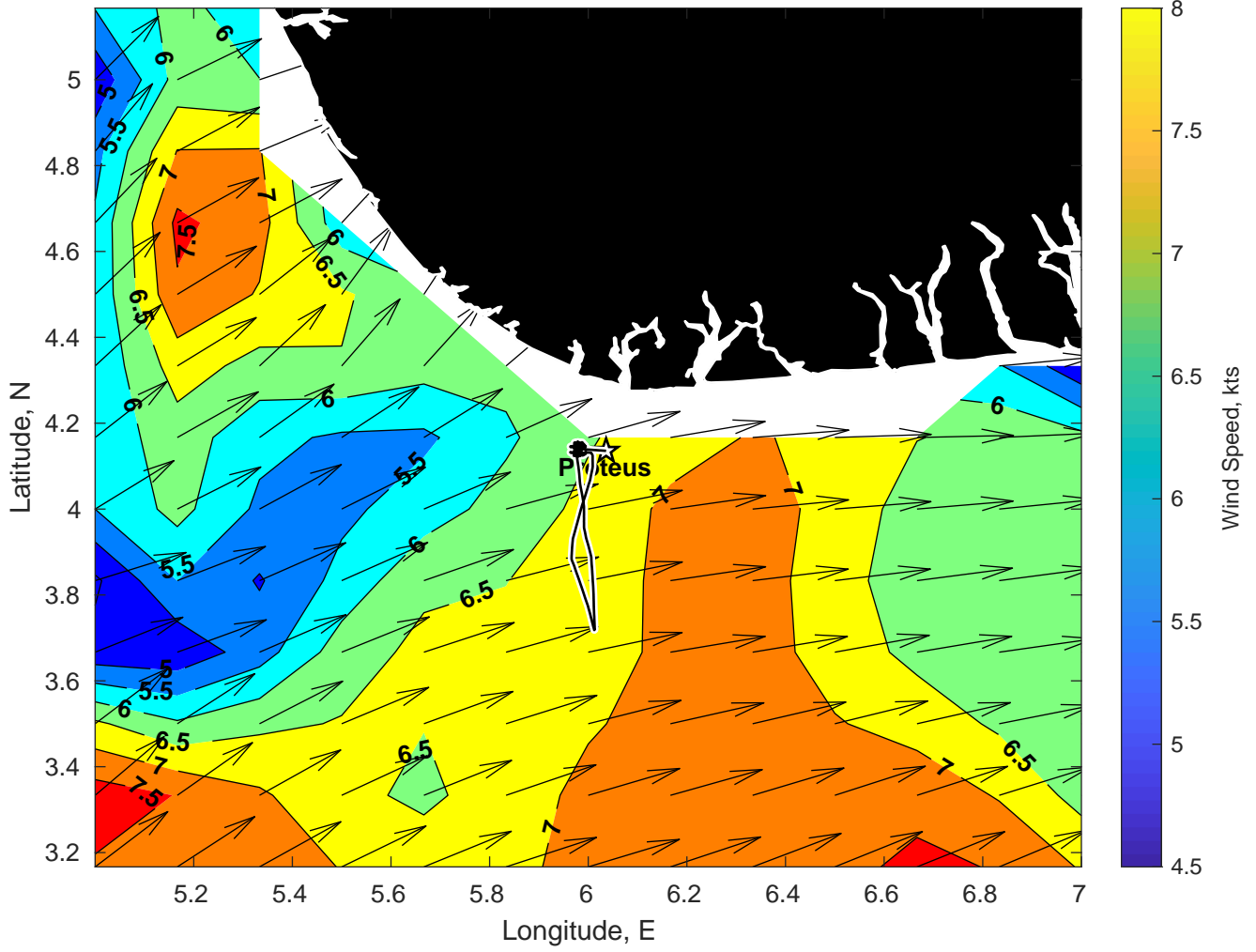
Winds (kts) for Proteus at 12-Feb-2025 09:00:00
