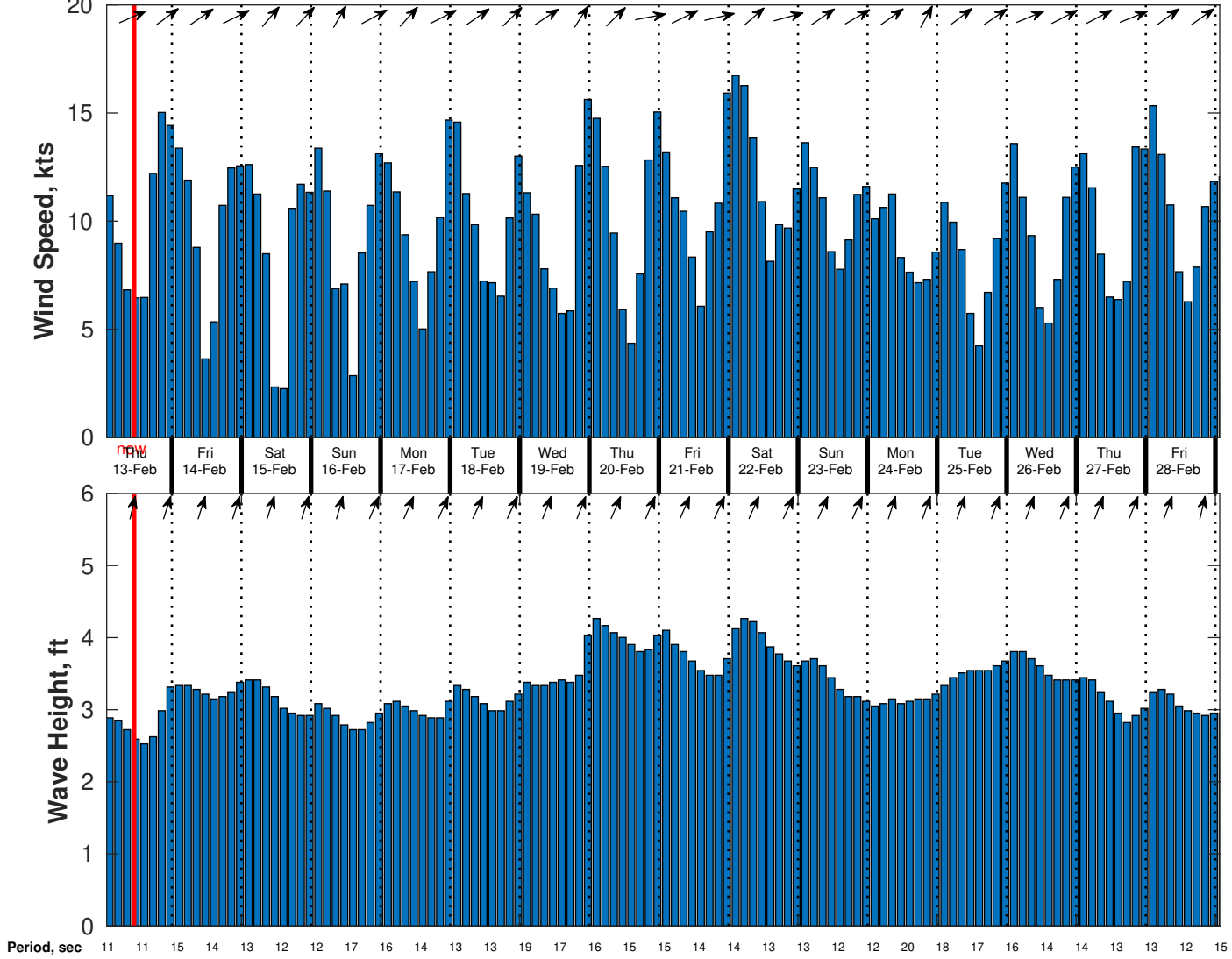
Wind & Wave Forecast for Proteus from 12-Feb-2025 01:00:00 to 28-Feb-2025 01:00:00
