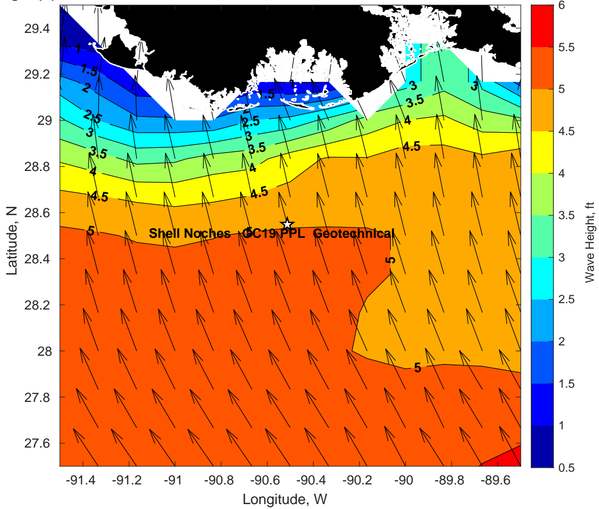
Wave Height (ft) for Shell Noches GC19 PPL Geotechnical at 12-Feb-2025 09:00:00
