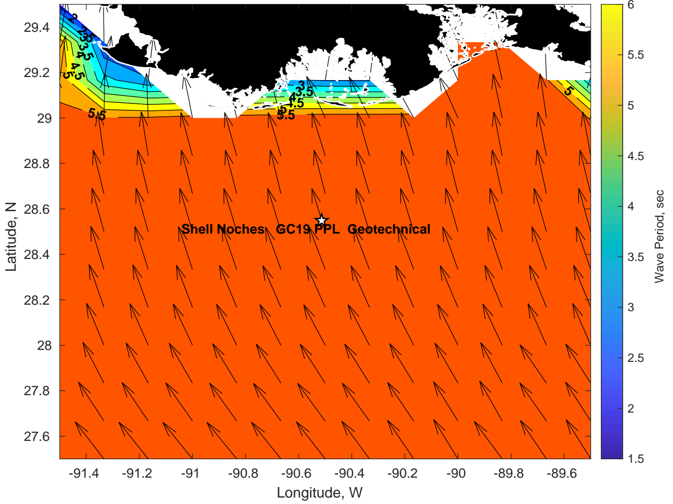
Wave Period (sec) for Shell Noches GC19 PPL Geotechnical at 12-Feb-2025 09:00:00
