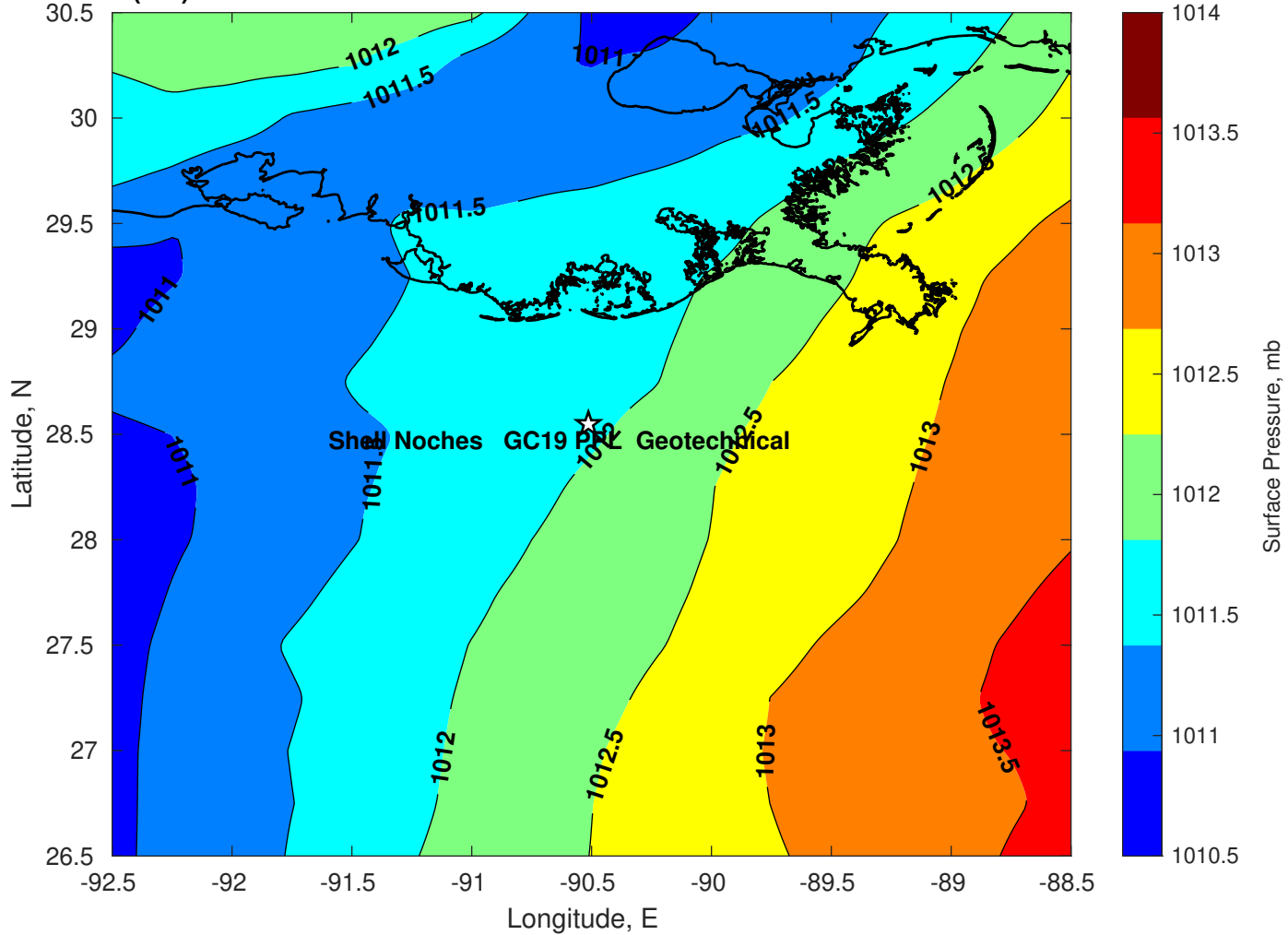
Surface Pressure (mb) for Shell Noches GC19 PPL Geotechnical at 12-Feb-2025 00:00:00
