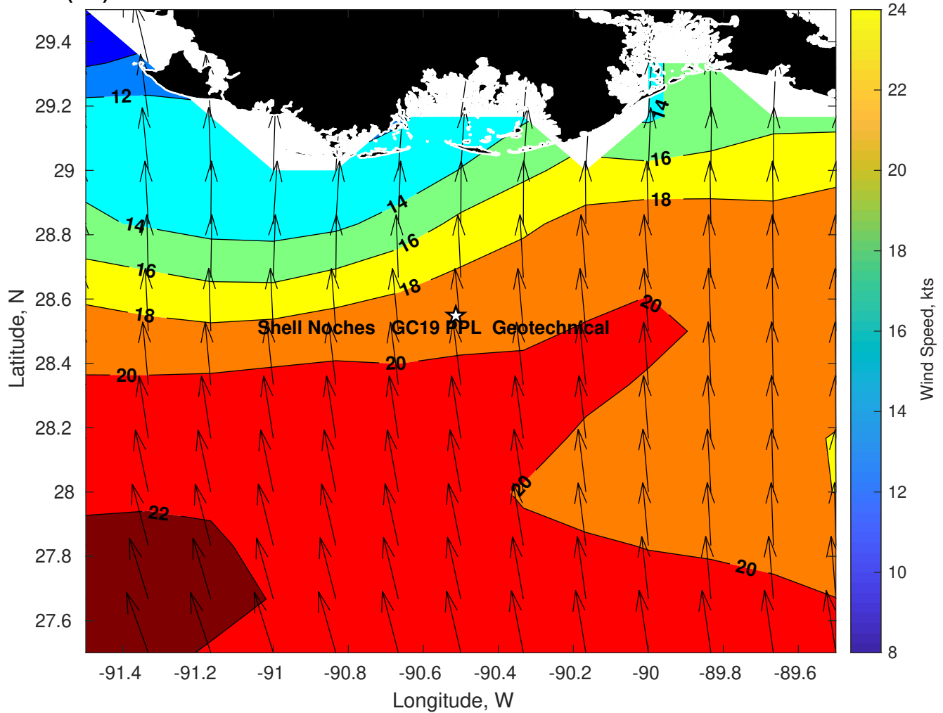
Winds (kts) for Shell Noches GC19 PPL Geotechnical at 12-Feb-2025 09:00:00
