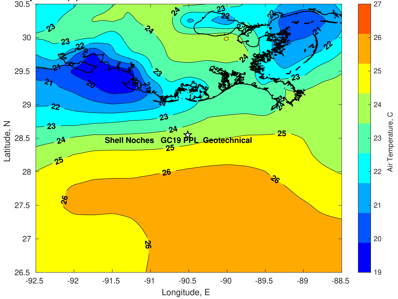
Air Temperature (C) for Shell Noches GC19 PPL Geotechnical at 12-Feb-2025
