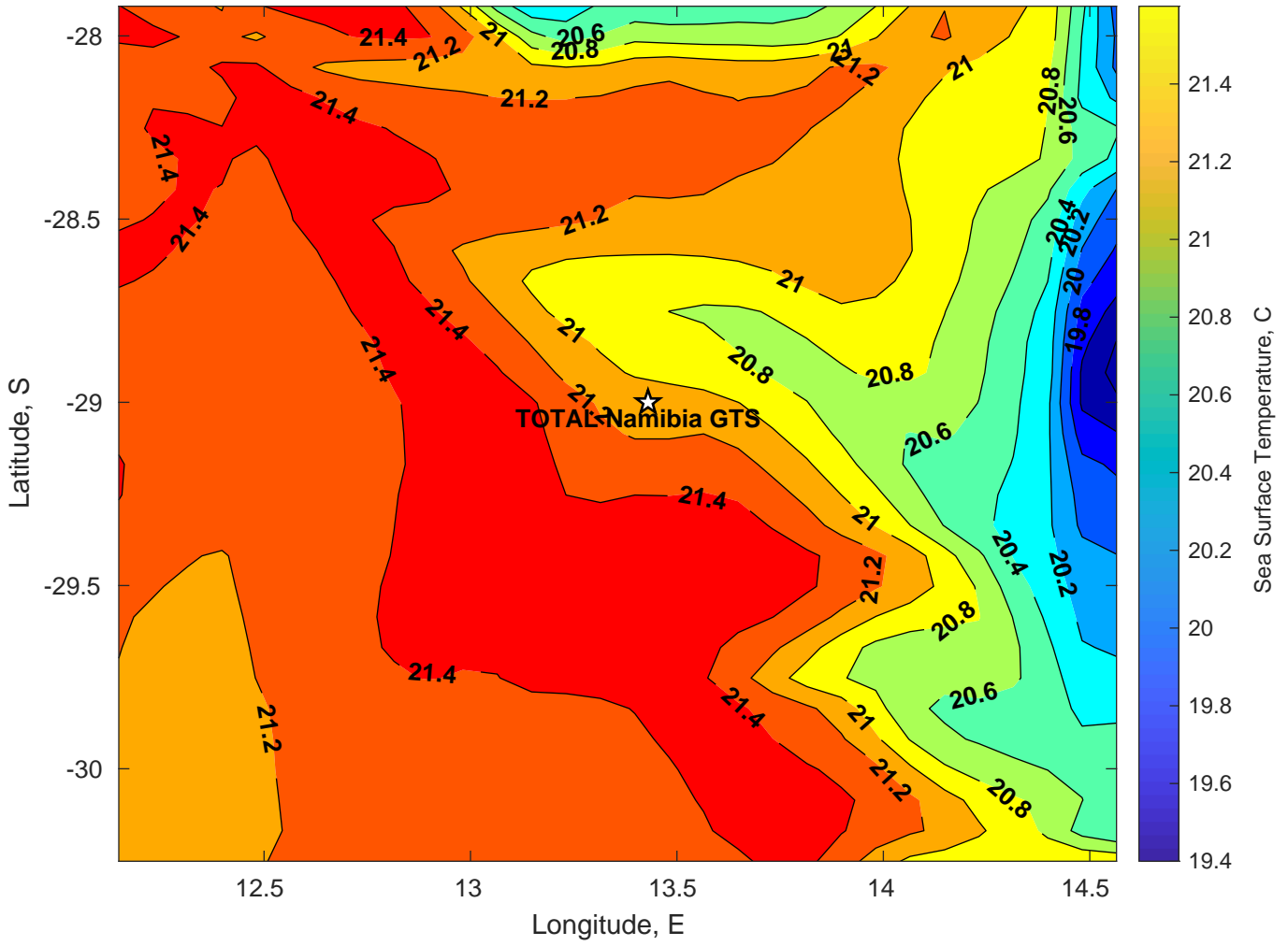
SST for TOTAL Namibia GTS at 11-Feb-2025 00:00:00
