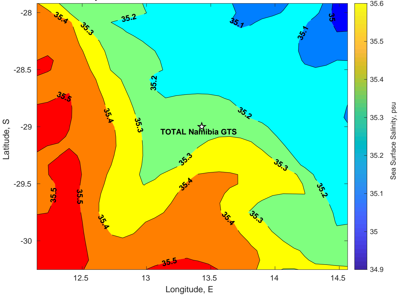
Surface Salinity for TOTAL Namibia GTS at 11-Feb-2025 00:00:00
