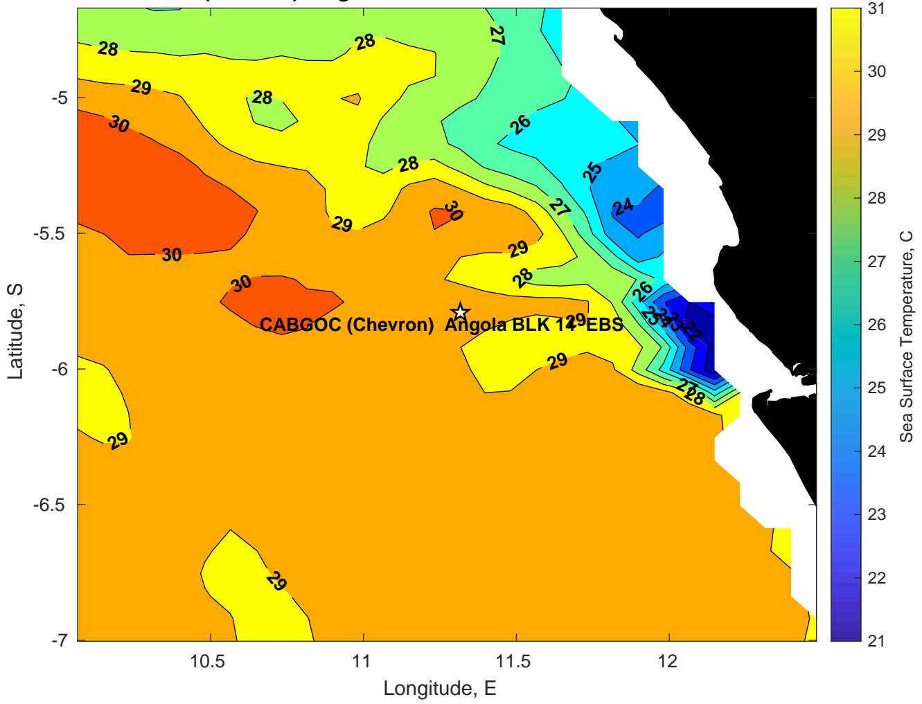
SST for CABGOC (Chevron) Angola BLK 14 EBS at 12-Feb-2025 00:00:00
