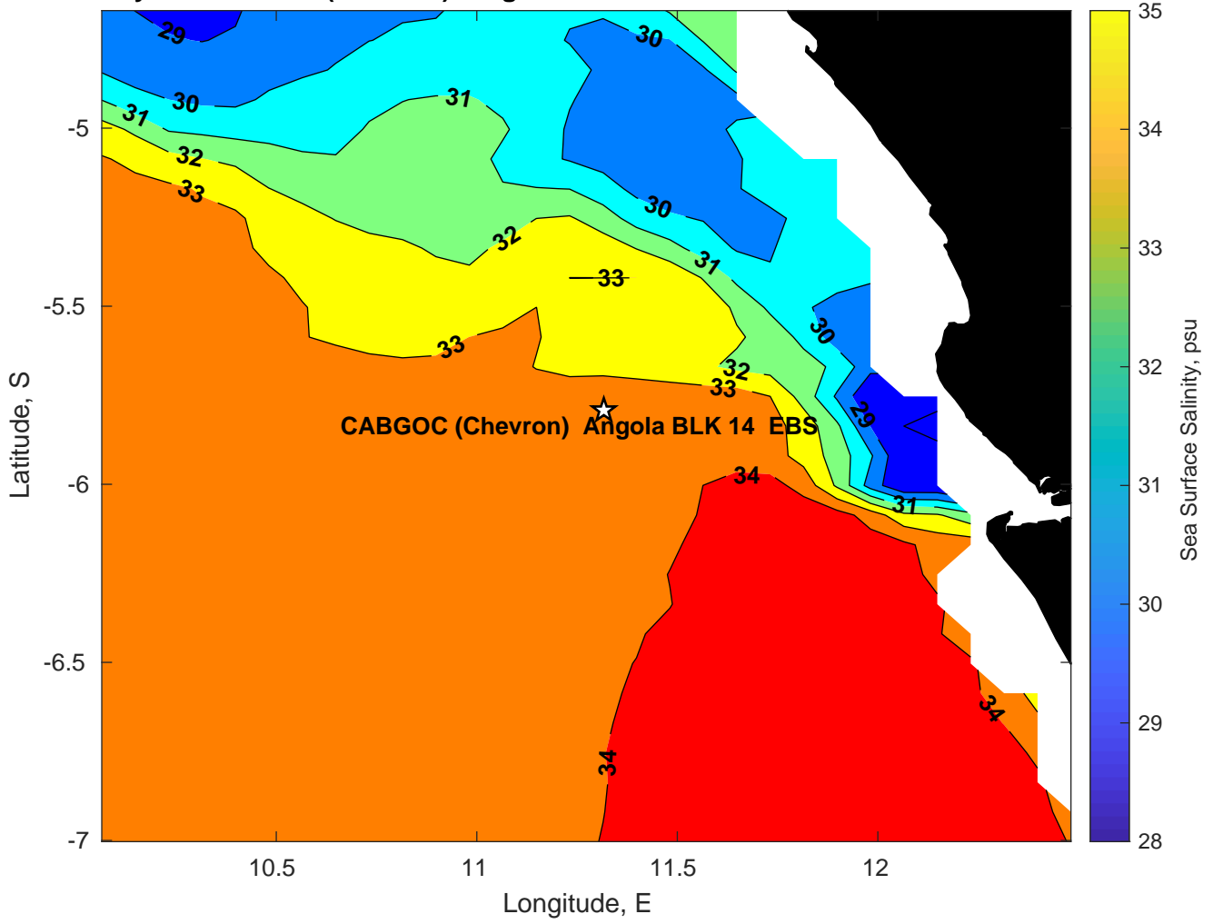
Surface Salinity for CABGOC (Chevron) Angola BLK 14 EBS at 12-Feb-2025 00:00:00
