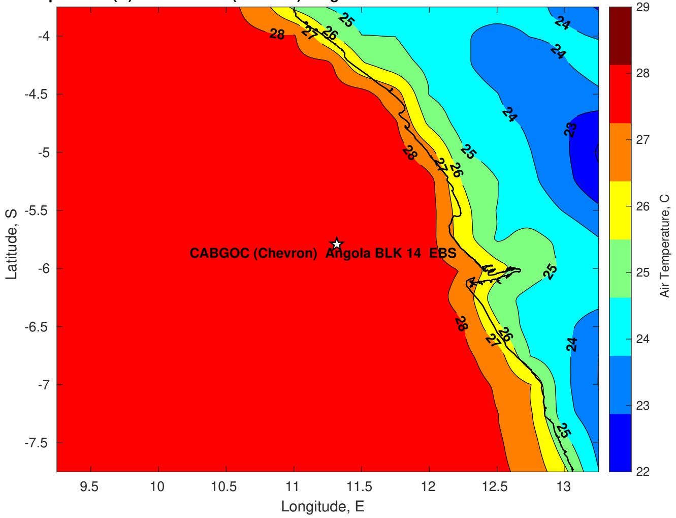
Air Temperature (C) for CABGOC (Chevron) Angola BLK 14 EBS at 13-Feb-2025
