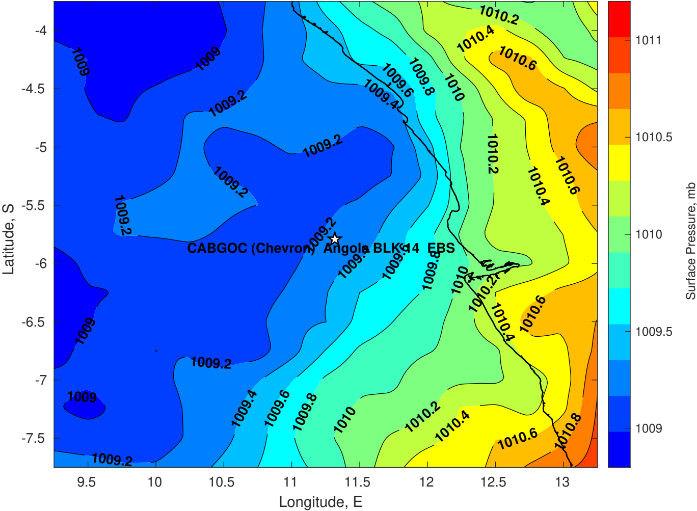
Surface Pressure (mb) for CABGOC (Chevron) Angola BLK 14 EBS at 13-Feb-2025 00:00:00
