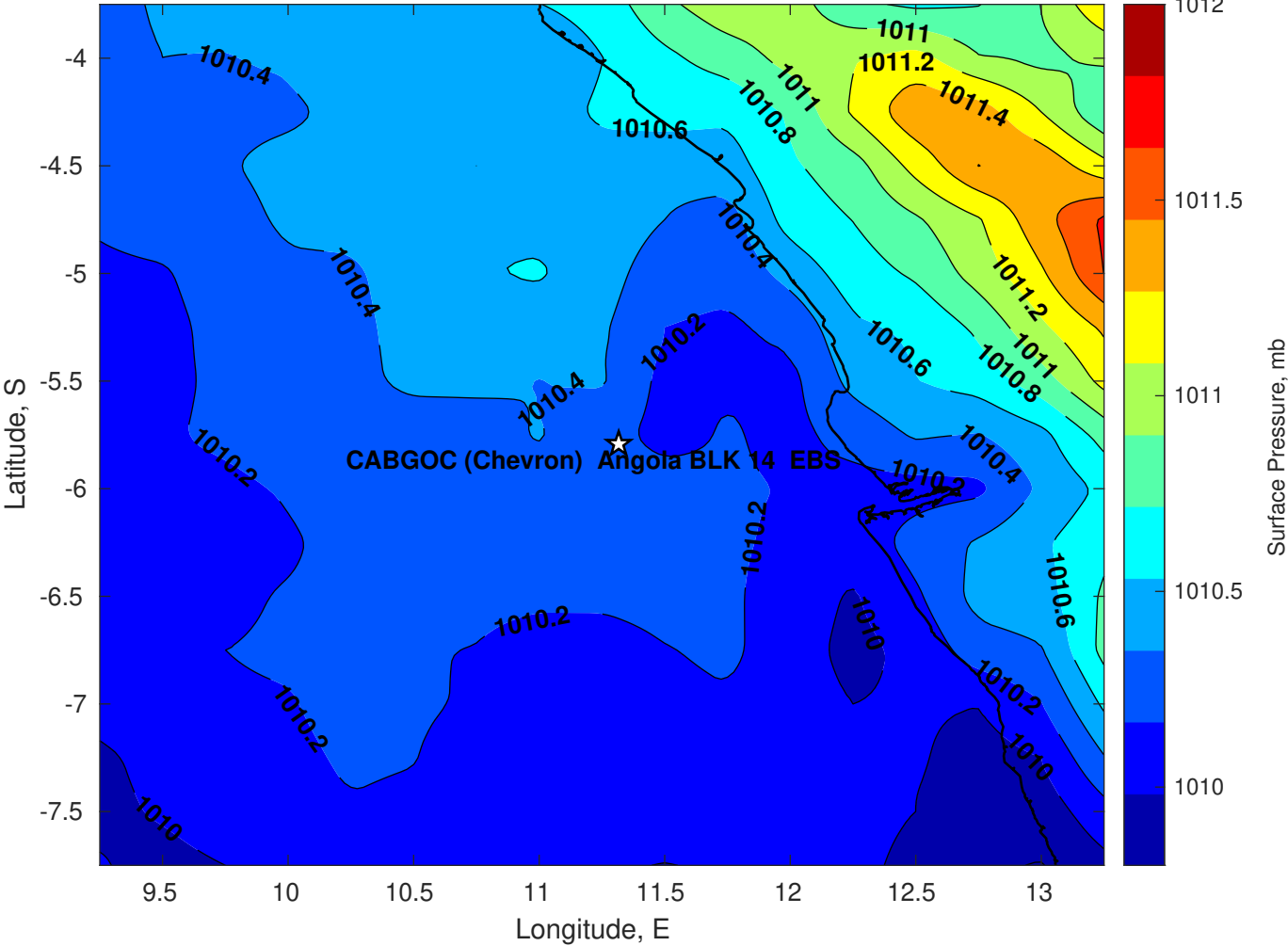
Surface Pressure (mb) for CABGOC (Chevron) Angola BLK 14 EBS at 14-Feb-2025 00:00:00
