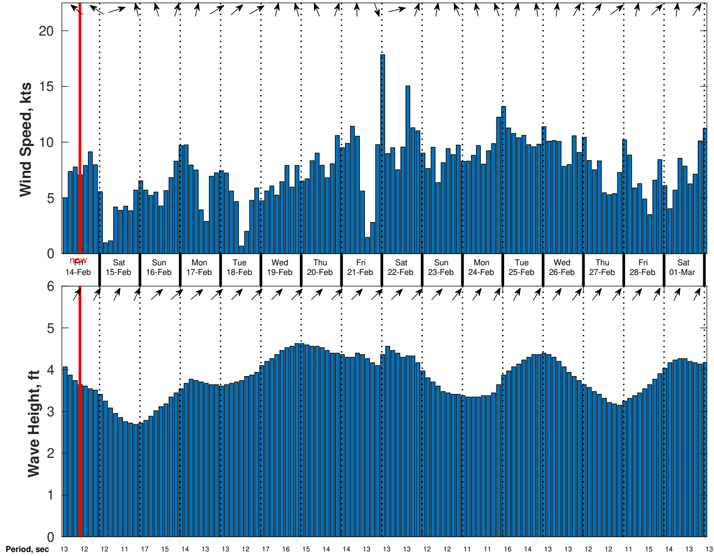
Wind & Wave Forecast for CABGOC (Chevron) Angola BLK 14 EBS from 13-Feb-2025 02:00:00 to 01-Mar-2025 02:00:00
