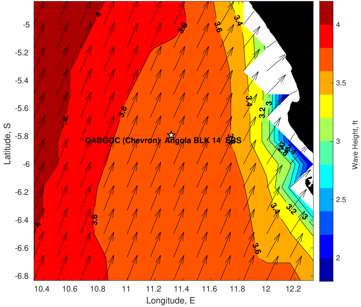
Wave Height (ft) for CABGOC (Chevron) Angola BLK 14 EBS at 13-Feb-2025 09:00:00
