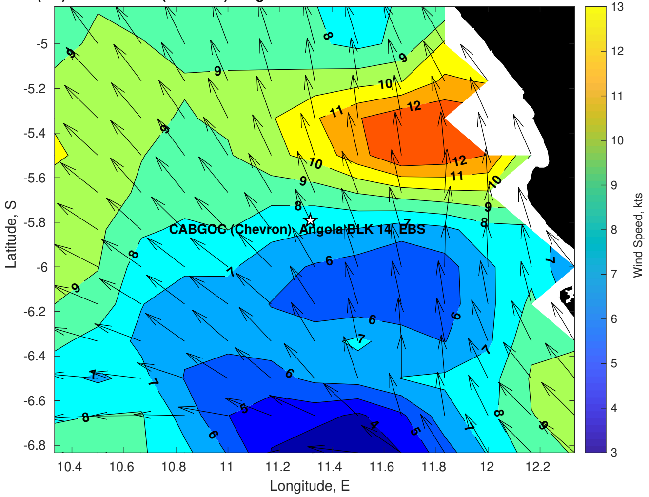
Winds (kts) for CABGOC (Chevron) Angola BLK 14 EBS at 13-Feb-2025 09:00:00
