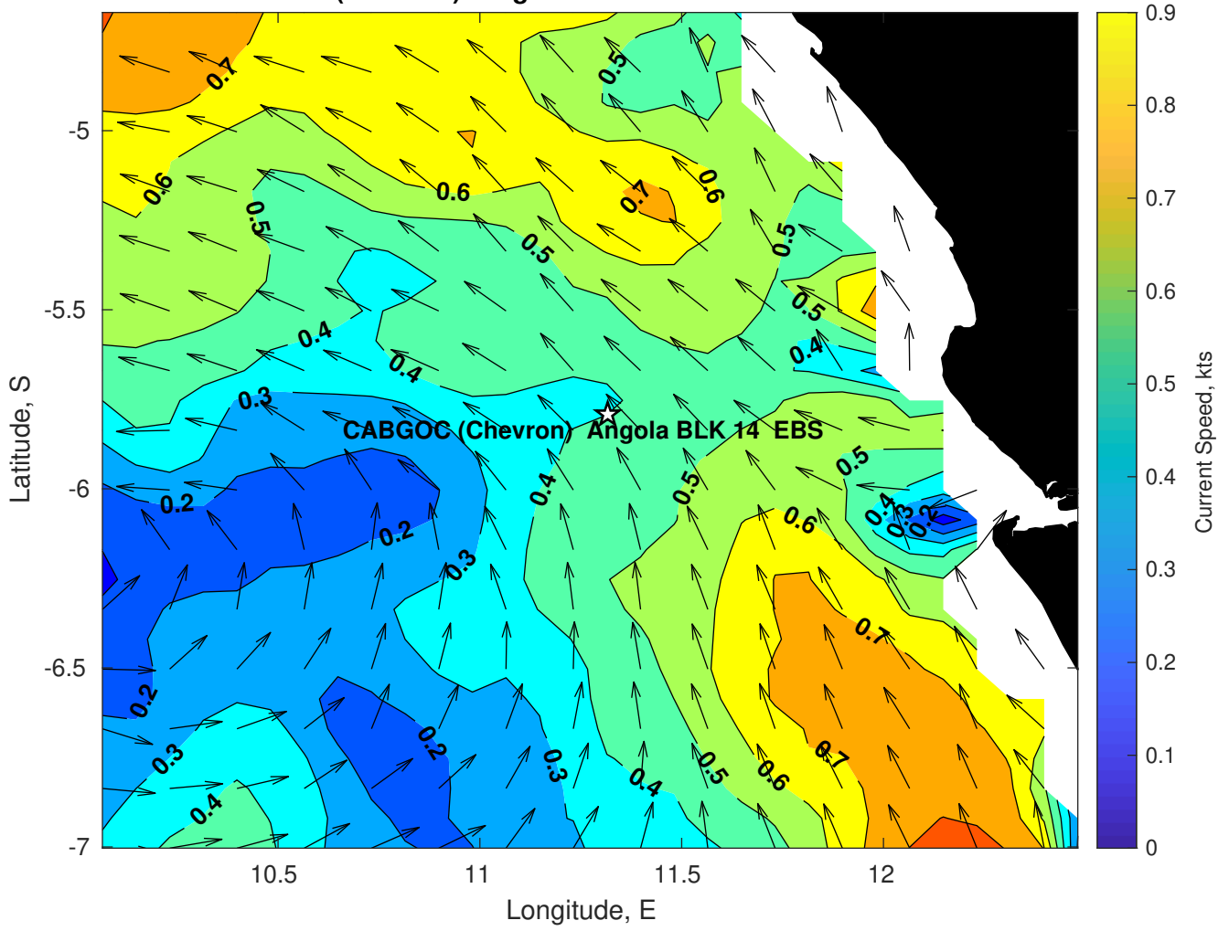
Surface Currents for CABGOC (Chevron) Angola BLK 14 EBS at 12-Feb-2025 00:00:00
