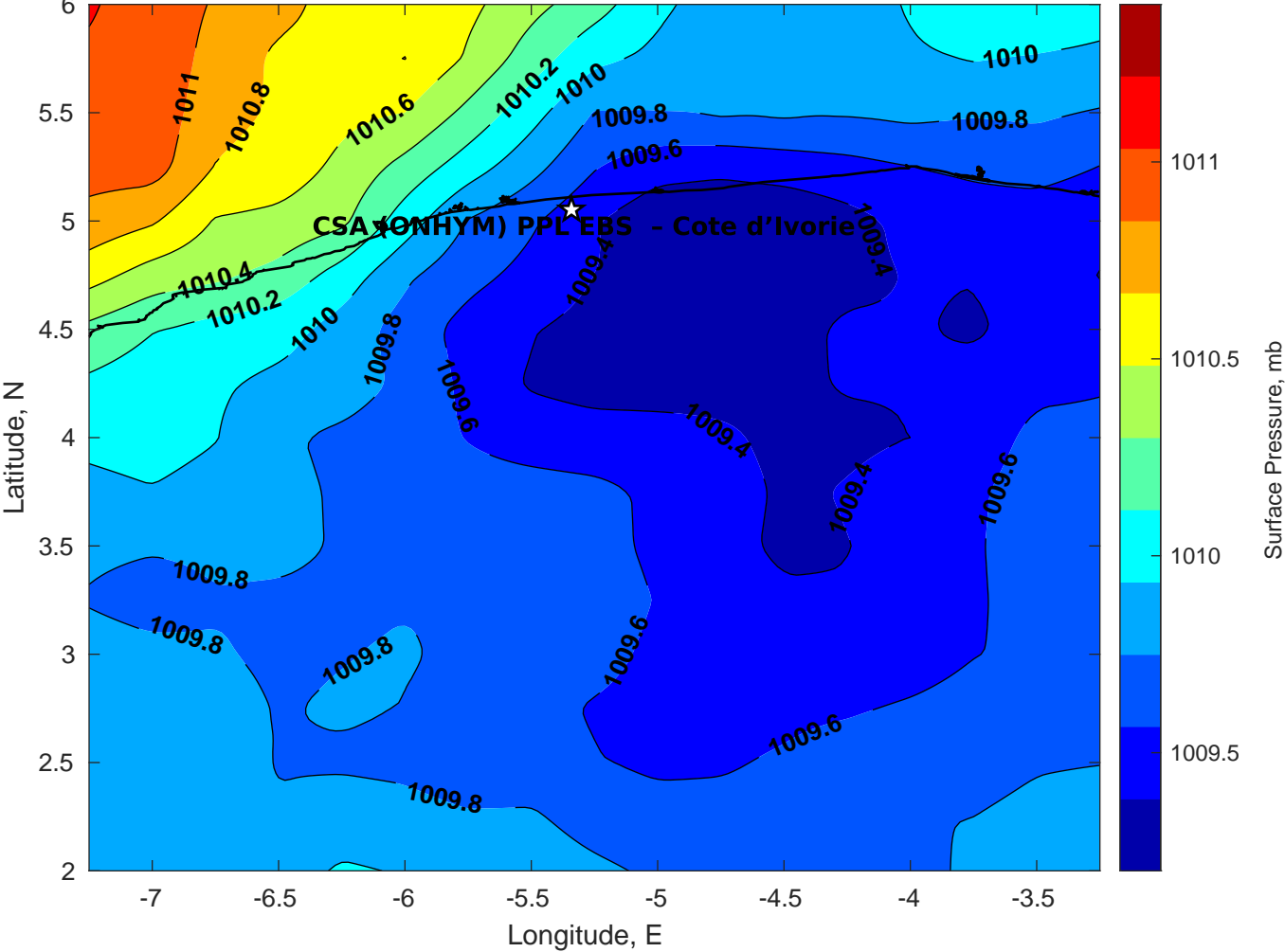
Surface Pressure (mb) for CSA (ONHYM) PPL EBS - Cote d'Ivoire at 13-Feb-2025 06:00:00
