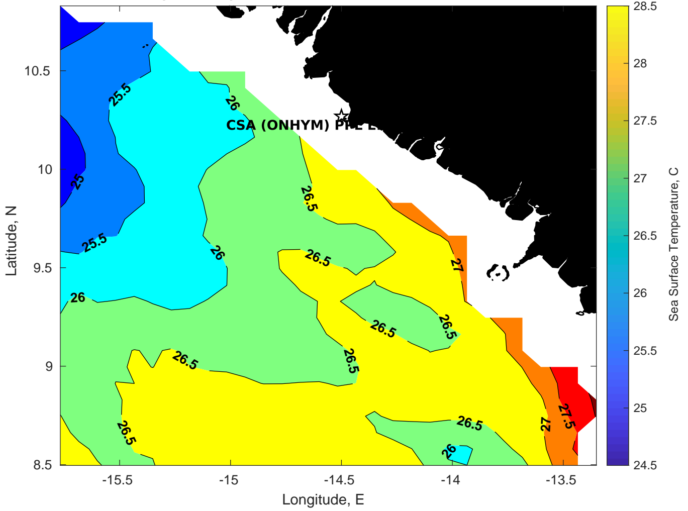
SST for CSA (ONHYM) PPL EBS - Guinea at 12-Feb-2025 00:00:00
