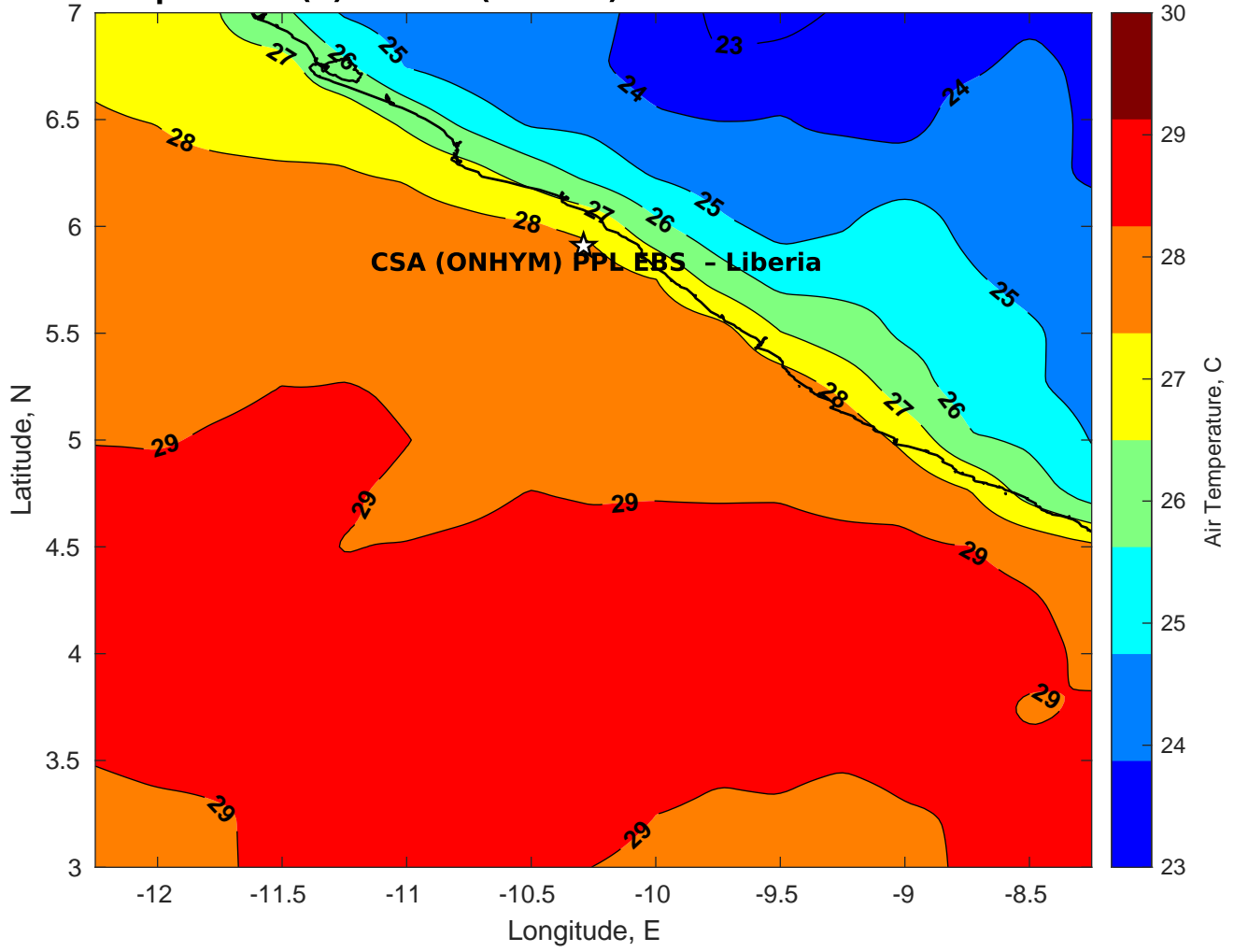
Air Temperature (C) for CSA (ONHYM) PPL EBS - Liberia at 13-Feb-2025
