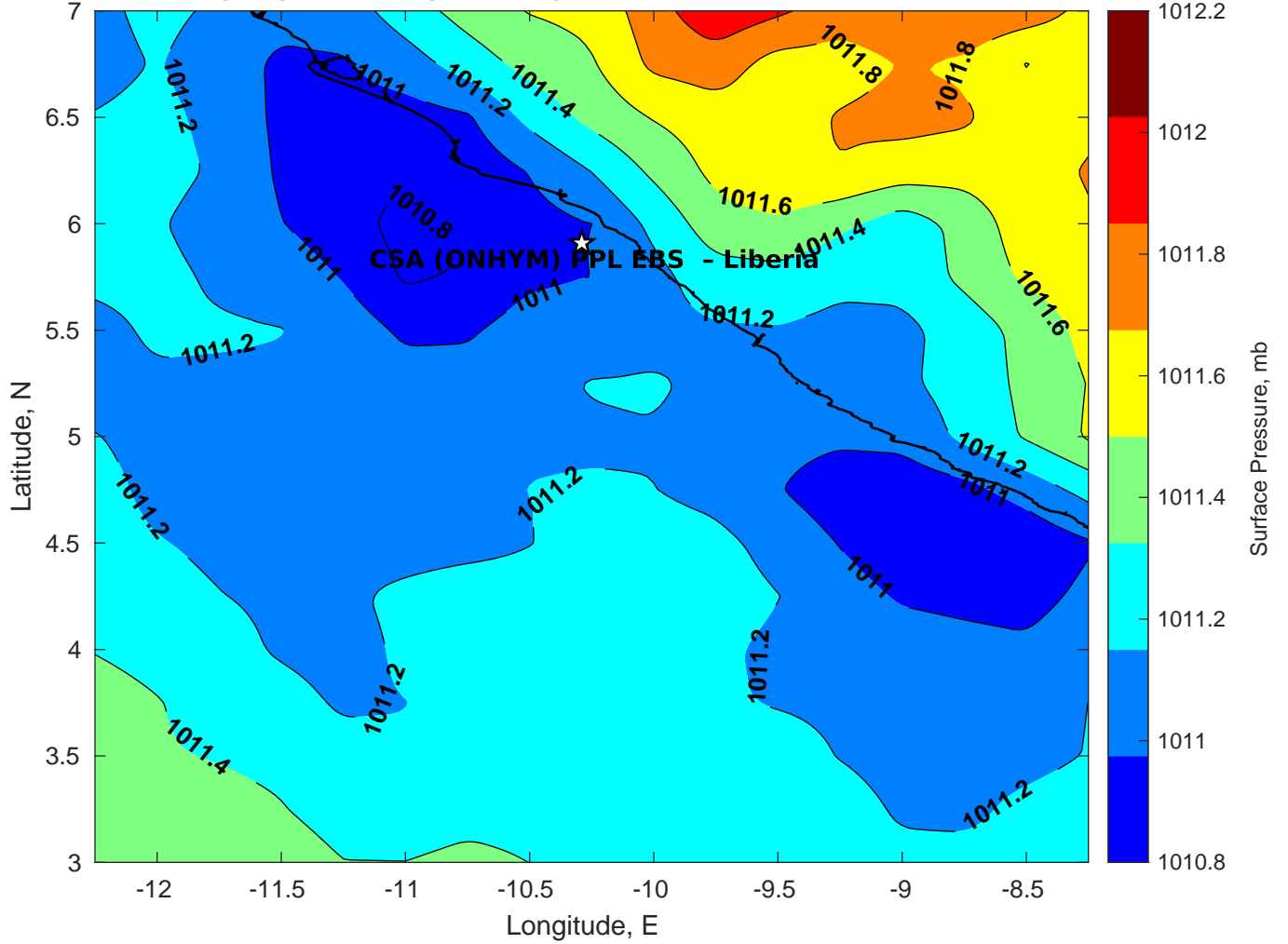
Surface Pressure (mb) for CSA (ONHYM) PPL EBS - Liberia at 13-Feb-2025 00:00:00
