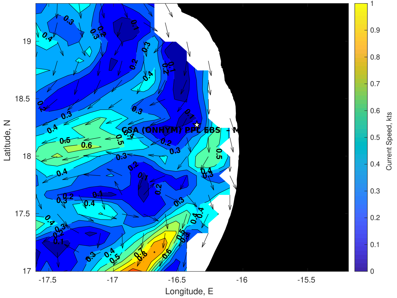
Surface Currents for CSA (ONHYM) PPL EBS - Mauritania at 12-Feb-2025 00:00:00
