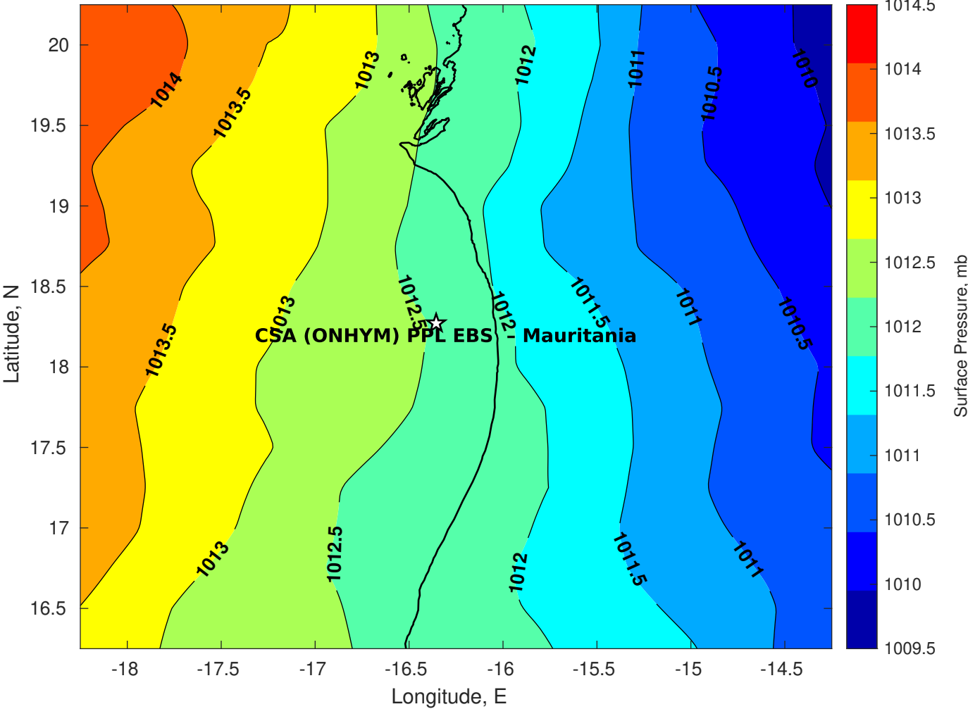
Surface Pressure (mb) for CSA (ONHYM) PPL EBS - Mauritania at 15-Feb-2025 00:00:00
