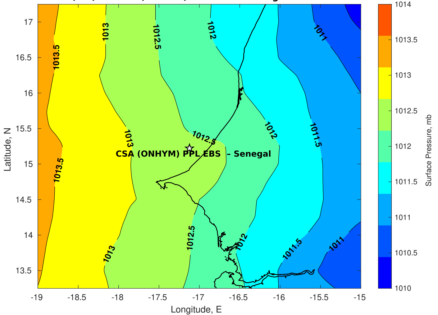
Surface Pressure (mb) for CSA (ONHYM) PPL EBS - Senegal at 14-Feb-2025 00:00:00
