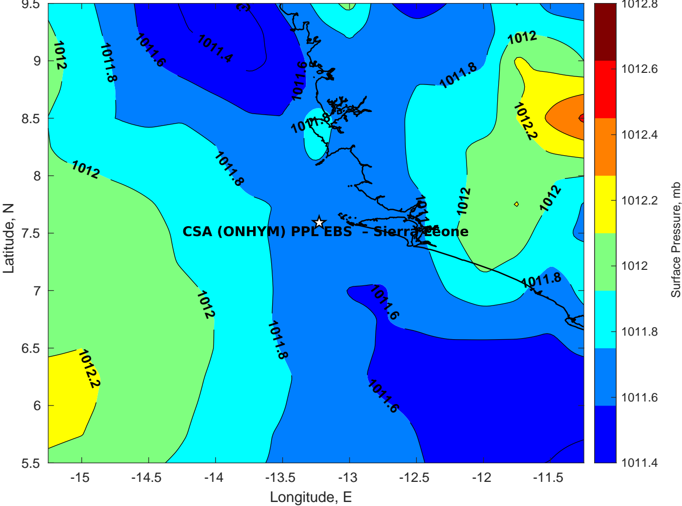
Surface Pressure (mb) for CSA (ONHYM) PPL EBS - Sierra Leone at 14-Feb-2025 00:00:00
