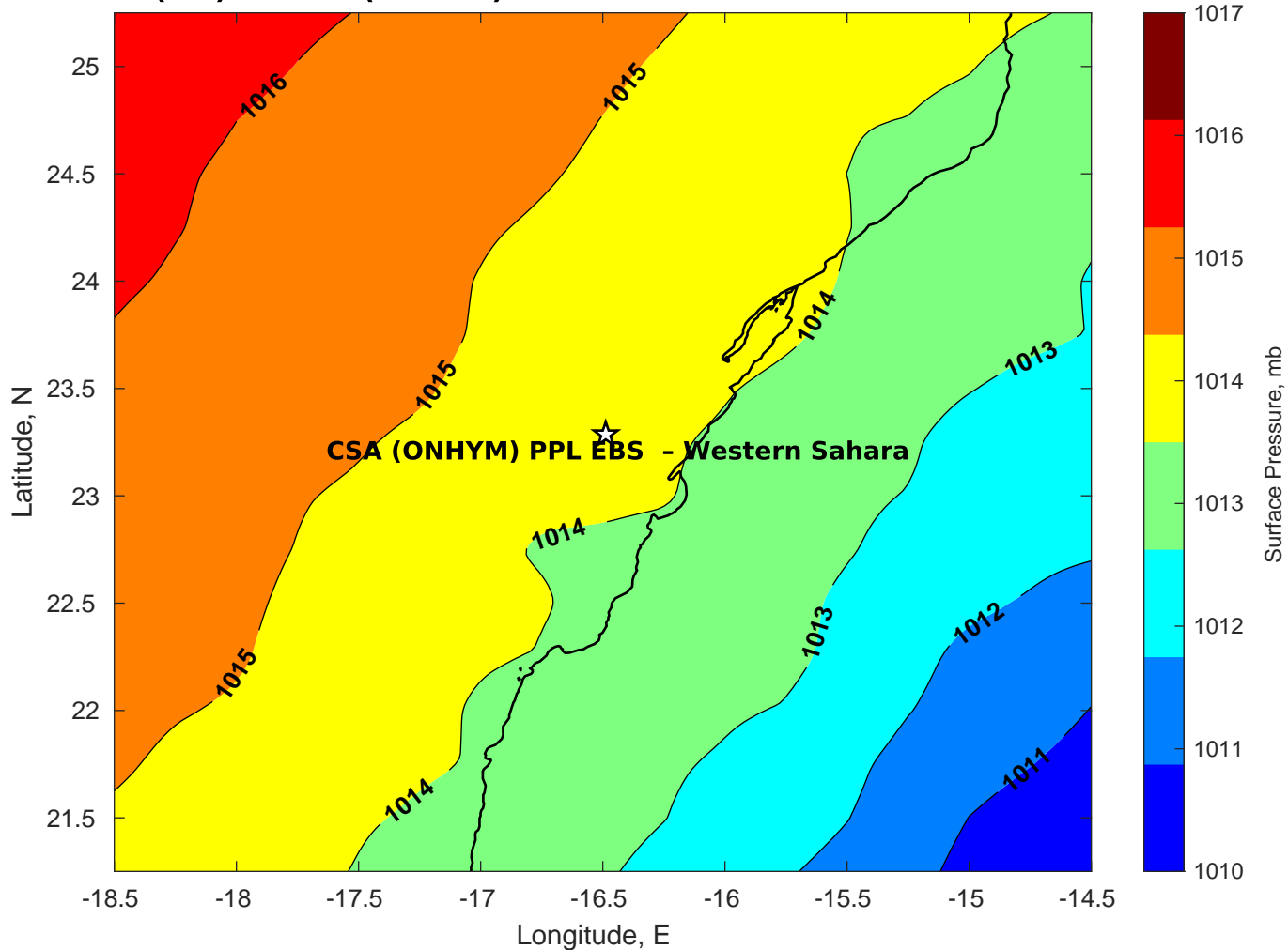
Surface Pressure (mb) for CSA (ONHYM) PPL EBS - Western Sahara at 15-Feb-2025 00:00:00
