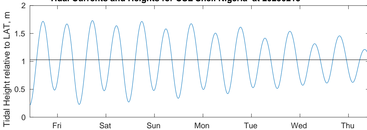
Tidal Currents and Heights for CSL Shell Nigeria at 20250213
