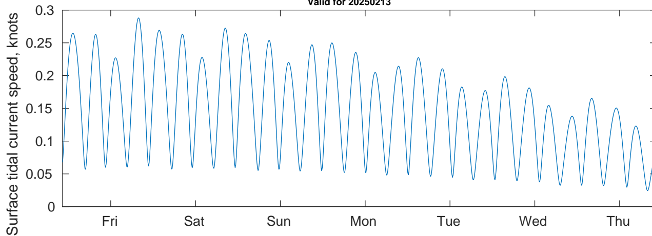
Tidal Currents and Heights for CSL Shell Nigeria at 20250213
