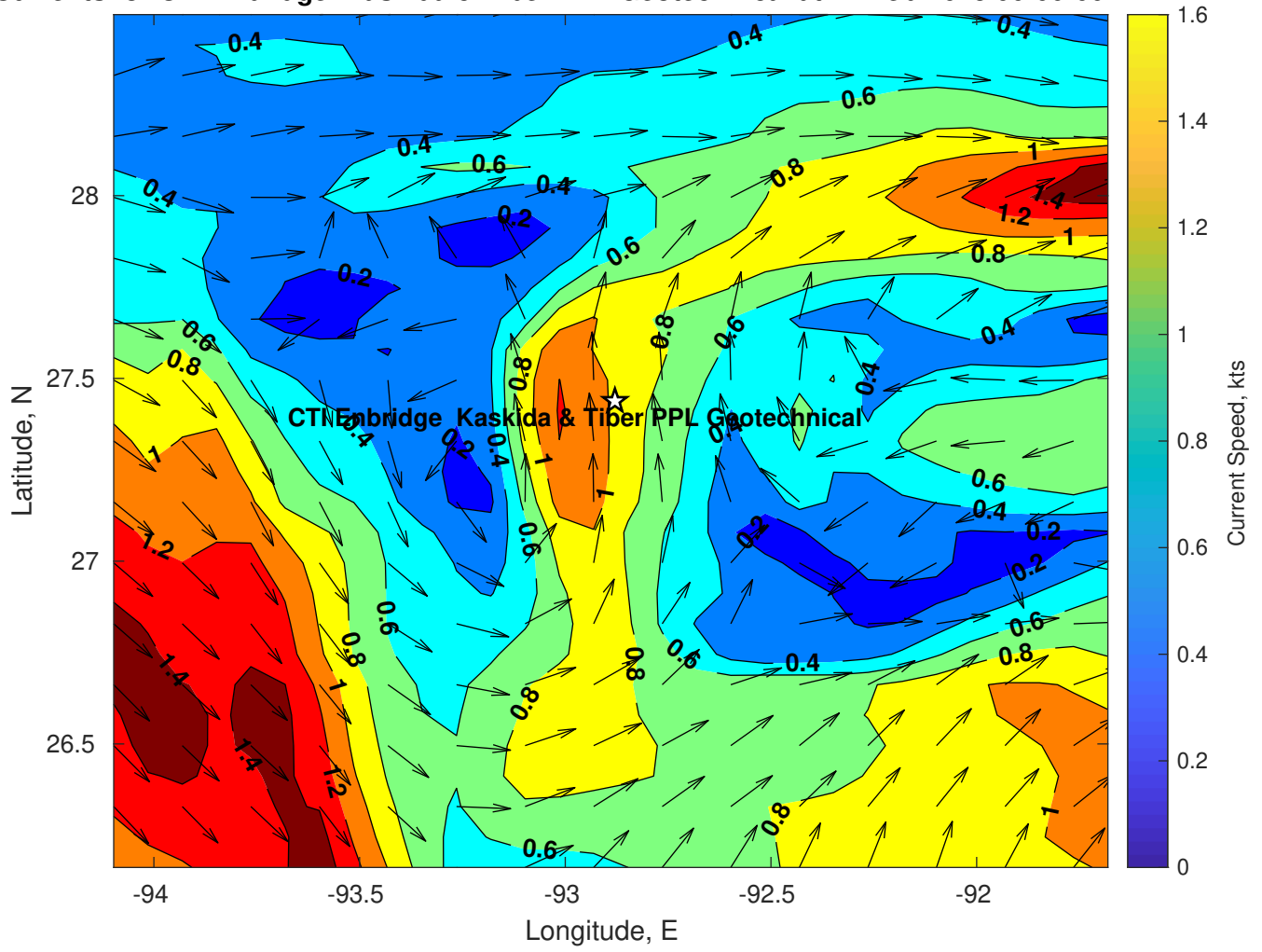
Surface Currents for CTI Enbridge Kaskida & Tiber PPL Geotechnical at 12-Feb-2025 00:00:00
