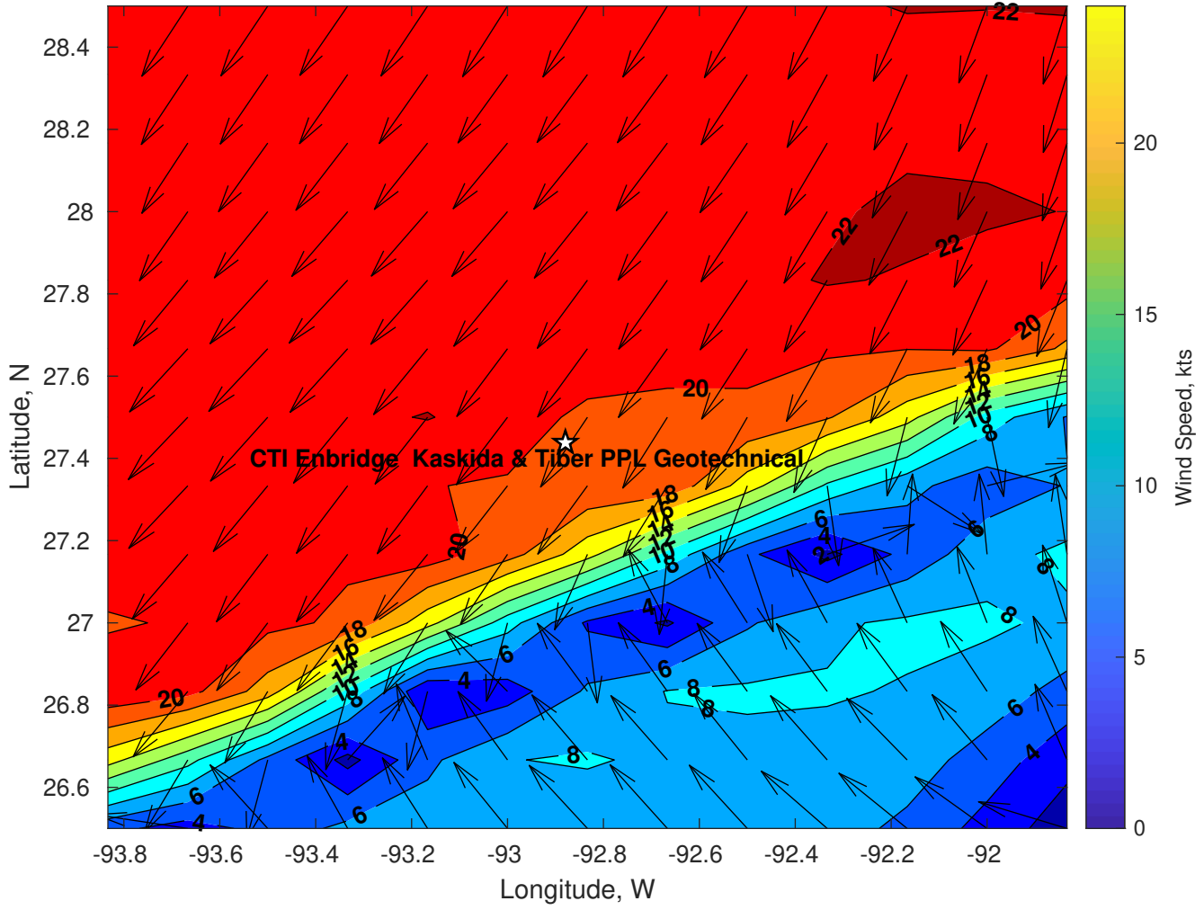
Winds (kts) for CTI Enbridge Kaskida & Tiber PPL Geotechnical at 13-Feb-2025 09:00:00
