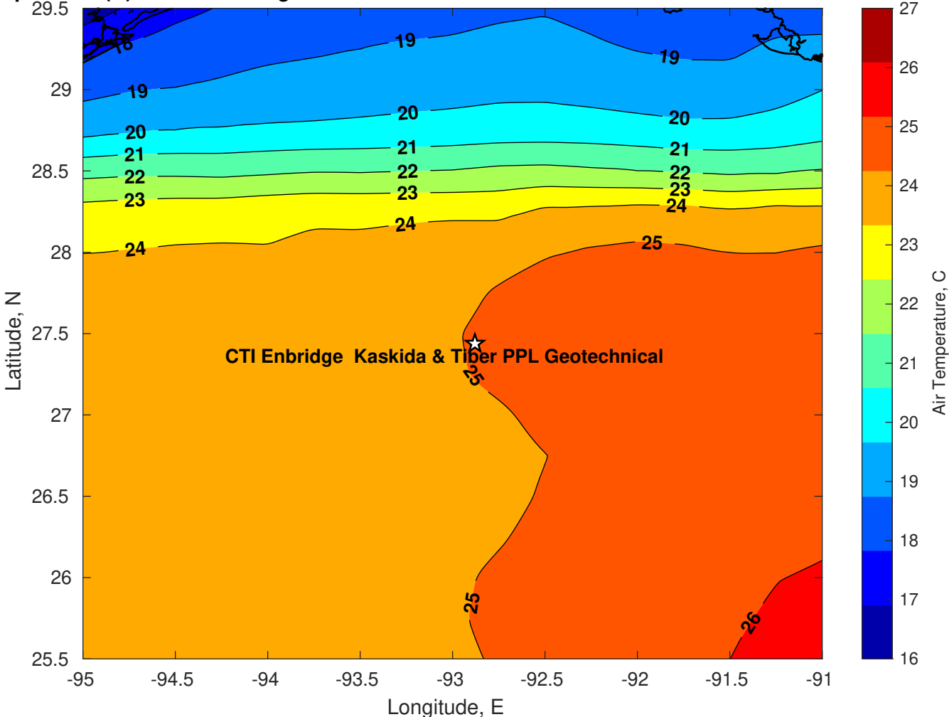
Air Temperature (C) for CTI Enbridge Kaskida & Tiber PPL Geotechnical at 13-Feb-2025
