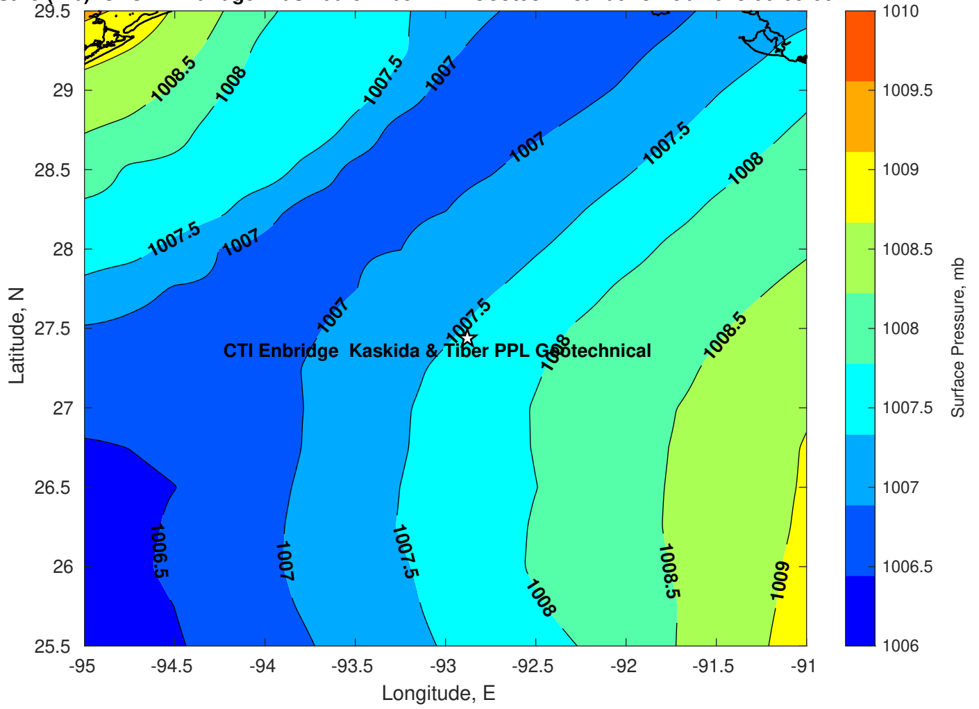
Surface Pressure (mb) for CTI Enbridge Kaskida & Tiber PPL Geotechnical at 13-Feb-2025 00:00:00
