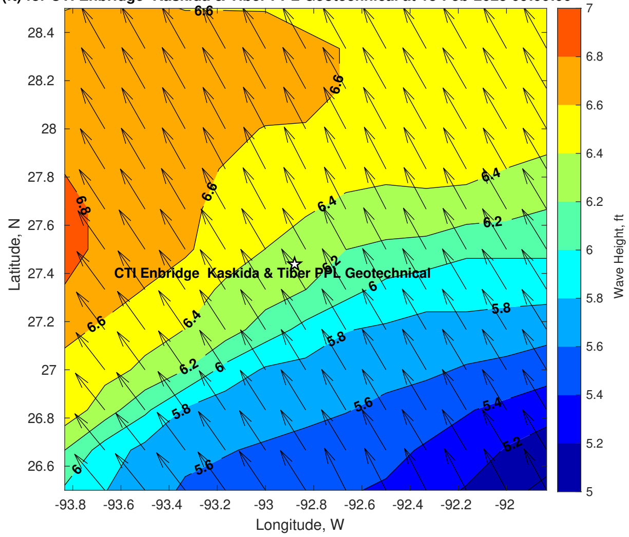
Wave Height (ft) for CTI Enbridge Kaskida & Tiber PPL Geotechnical at 13-Feb-2025 09:00:00
