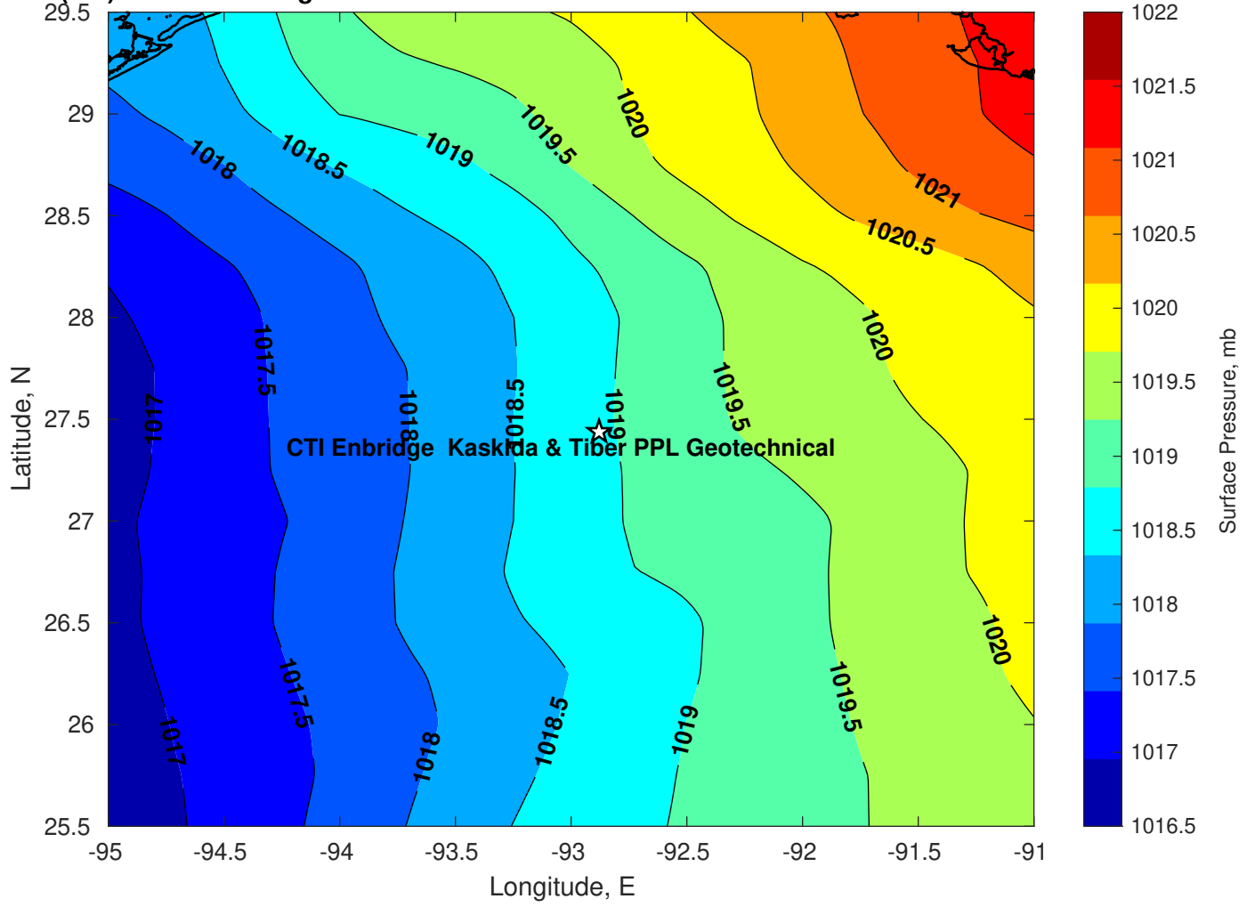
Surface Pressure (mb) for CTI Enbridge Kaskida & Tiber PPL Geotechnical at 15-Feb-2025 00:00:00
