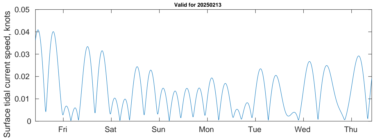
Tidal Currents and Heights for CTI Enbridge Kaskida & Tiber PPL Geotechnical at 20250213
