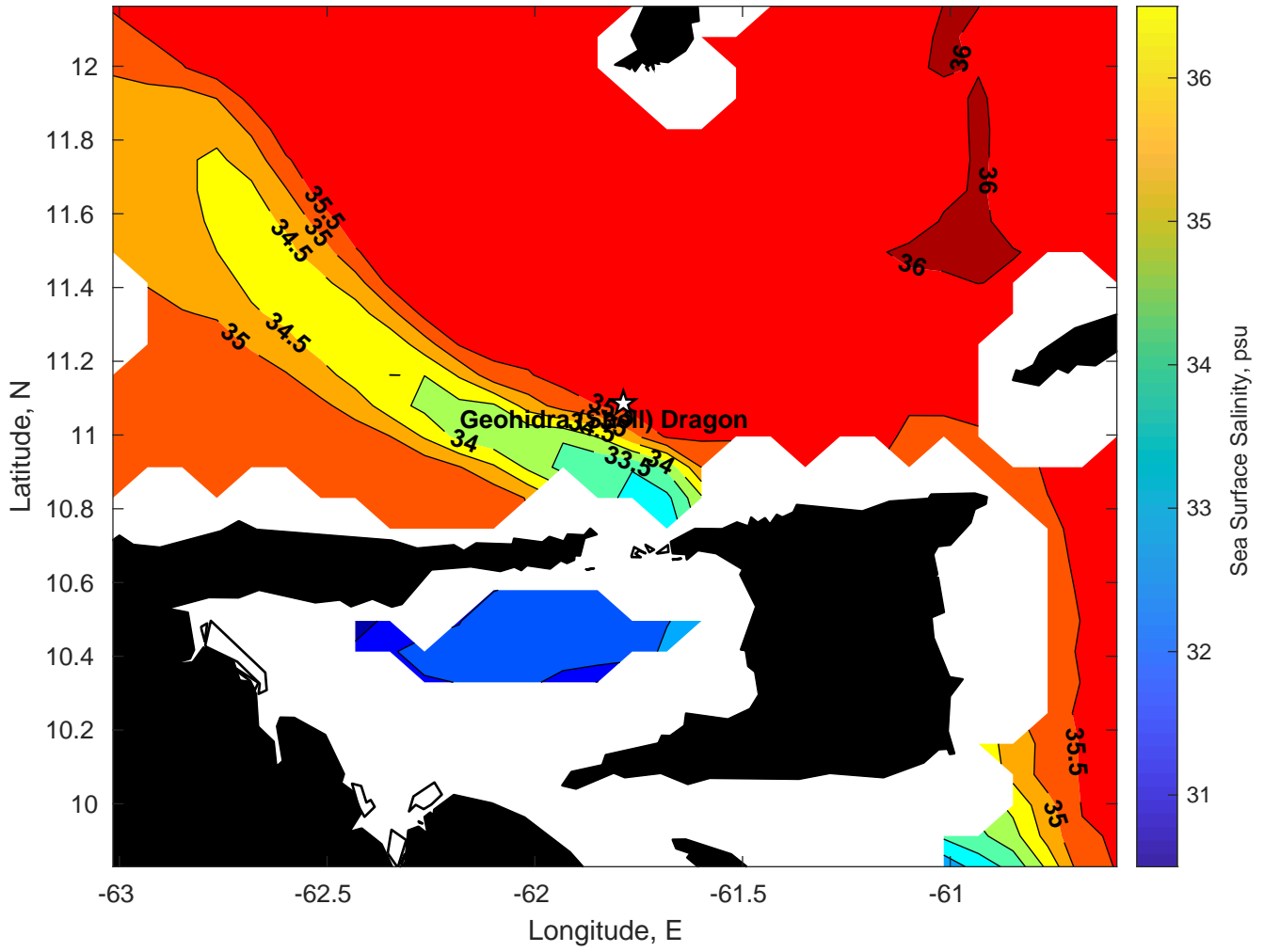
Surface Salinity for Geohdra (Shell) Dragon at 12-Feb-2025 00:00:00
