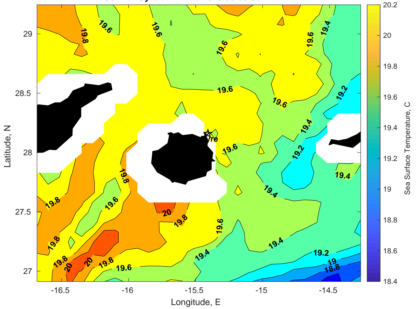
SST for Gyre at 12-Feb-2025 00:00:00
