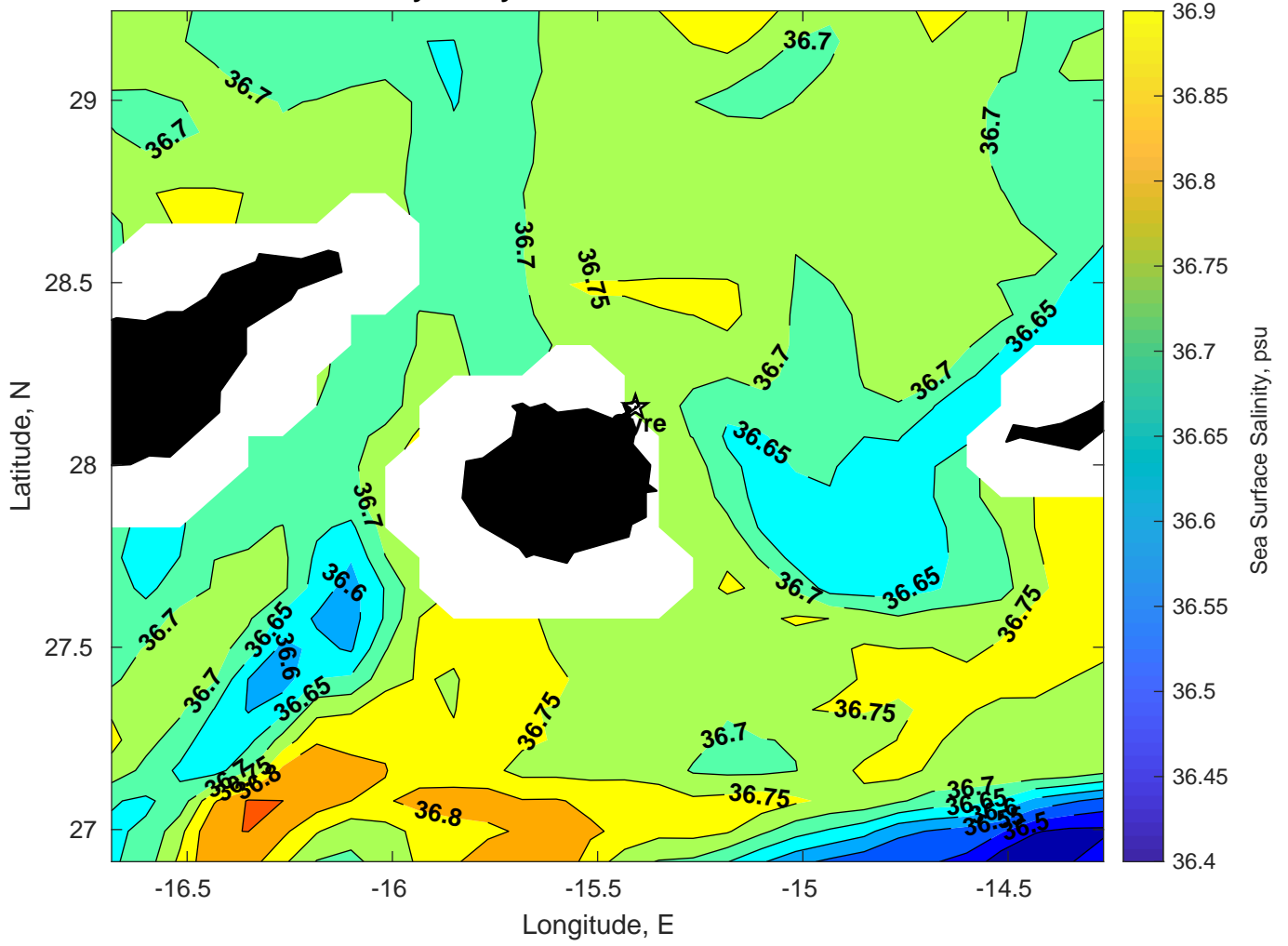
Surface Salinity for Gyre at 12-Feb-2025 00:00:00
