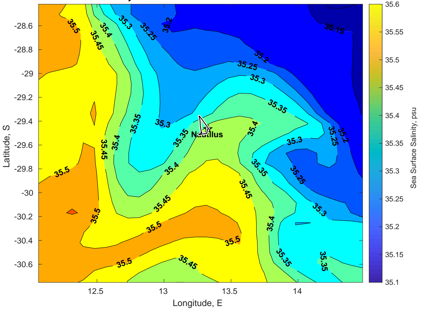
Surface Salinity for Nautilus at 12-Feb-2025 00:00:00
