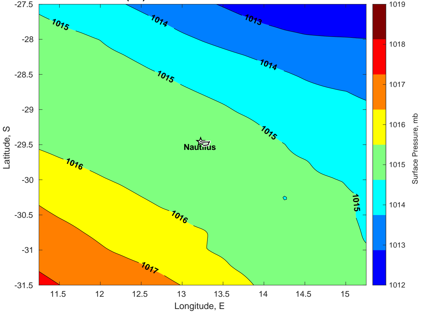
Surface Pressure (mb) for Nautilus at 13-Feb-2025 00:00:00
