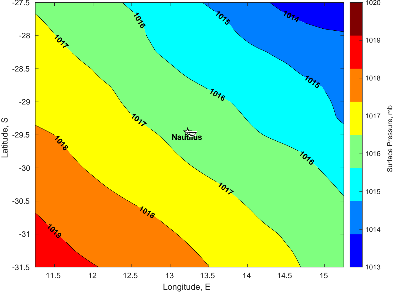
Surface Pressure (mb) for Nautilus at 14-Feb-2025 00:00:00
