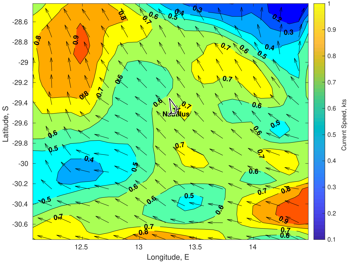
Surface Currents for Nautilus at 12-Feb-2025 00:00:00
