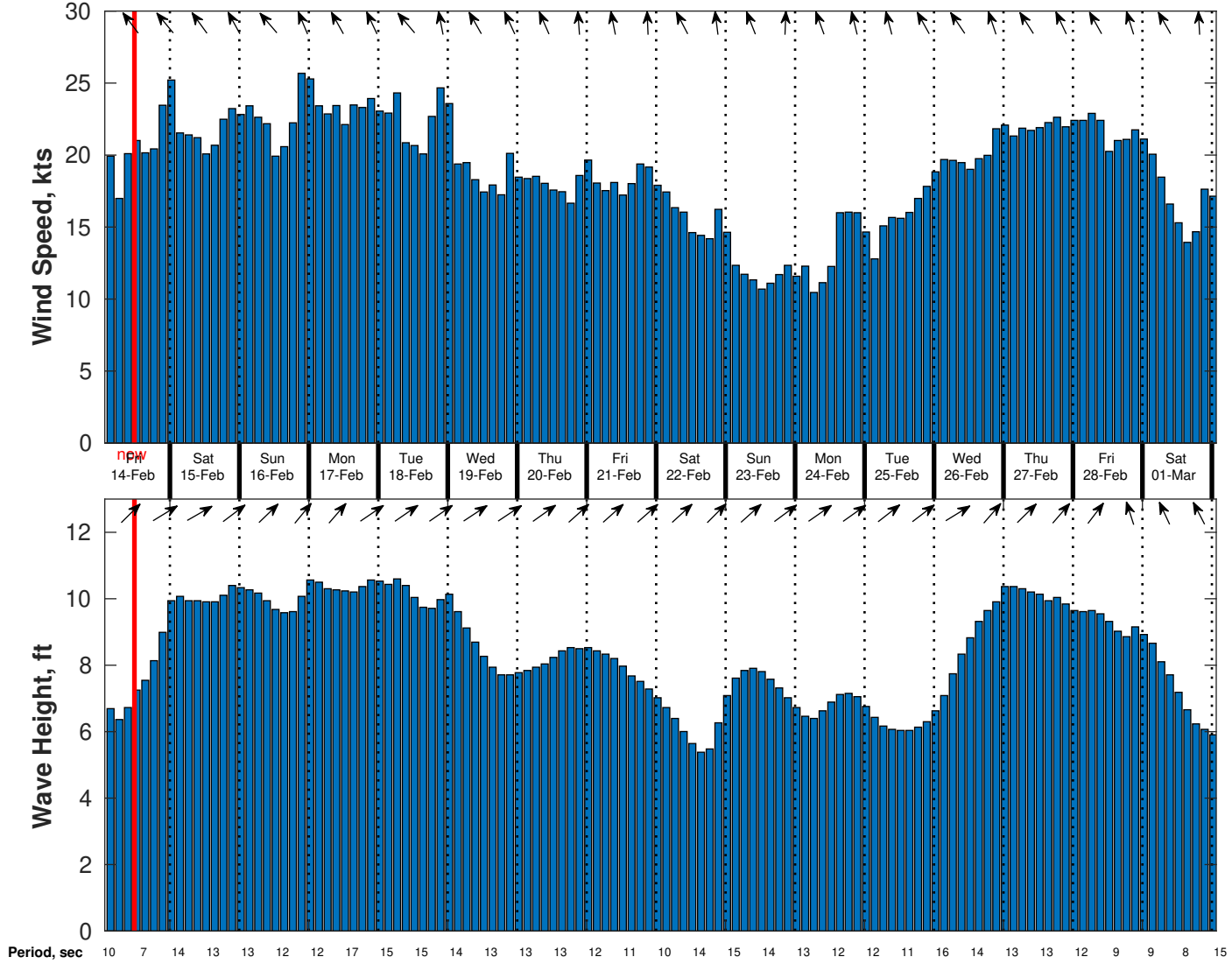
Wind & Wave Forecast for Nautilus from 13-Feb-2025 02:00:00 to 01-Mar-2025 02:00:00
