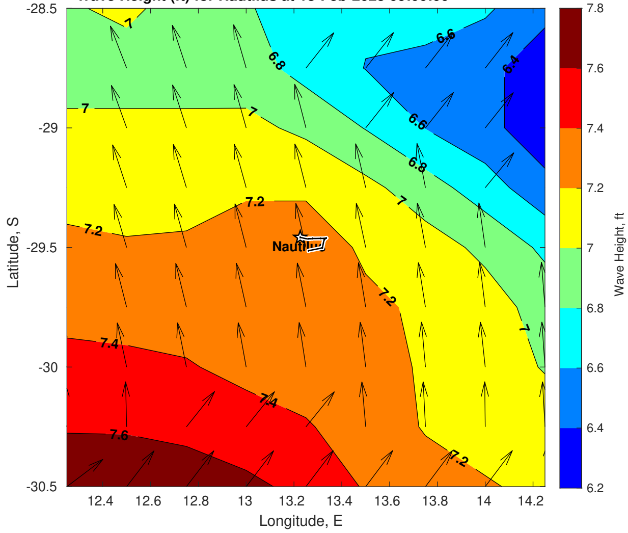
Wave Height (ft) for Nautilus at 13-Feb-2025 09:00:00
