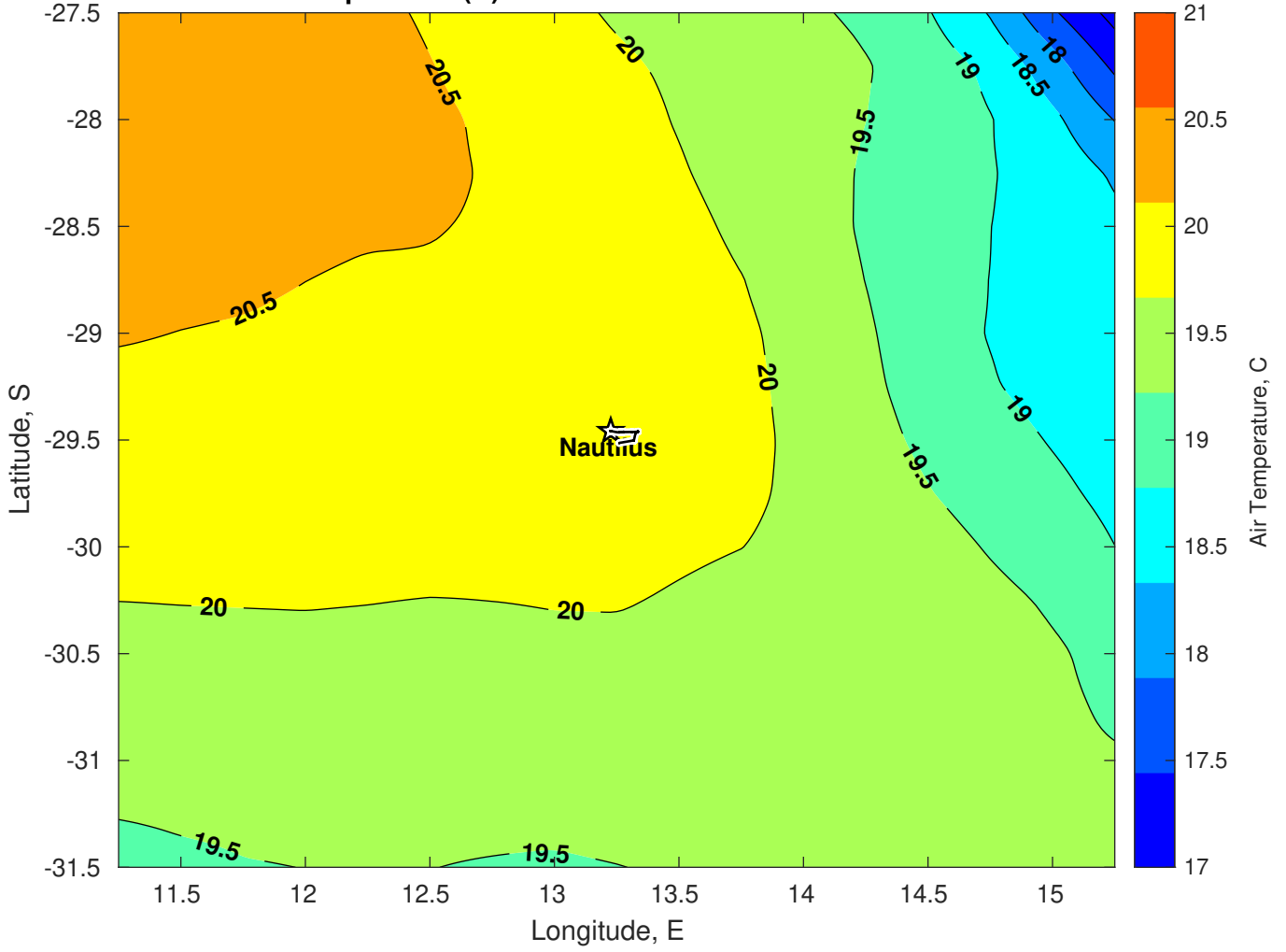
Air Temperature (C) for Nautilus at 13-Feb-2025
