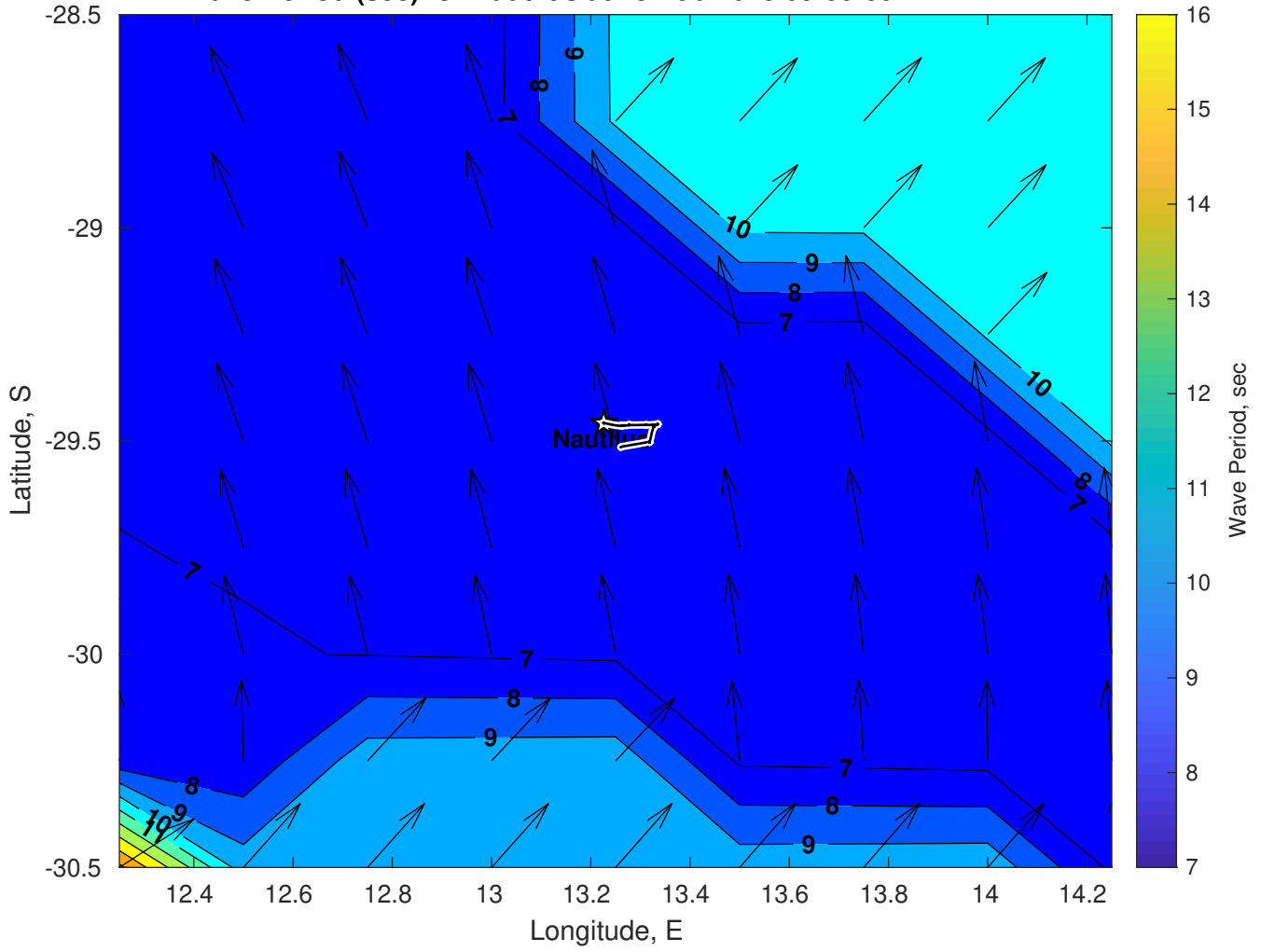
Wave Period (sec) for Nautilus at 13-Feb-2025 09:00:00
