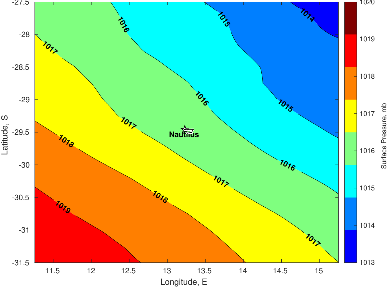
Surface Pressure (mb) for Nautilus at 15-Feb-2025 00:00:00
