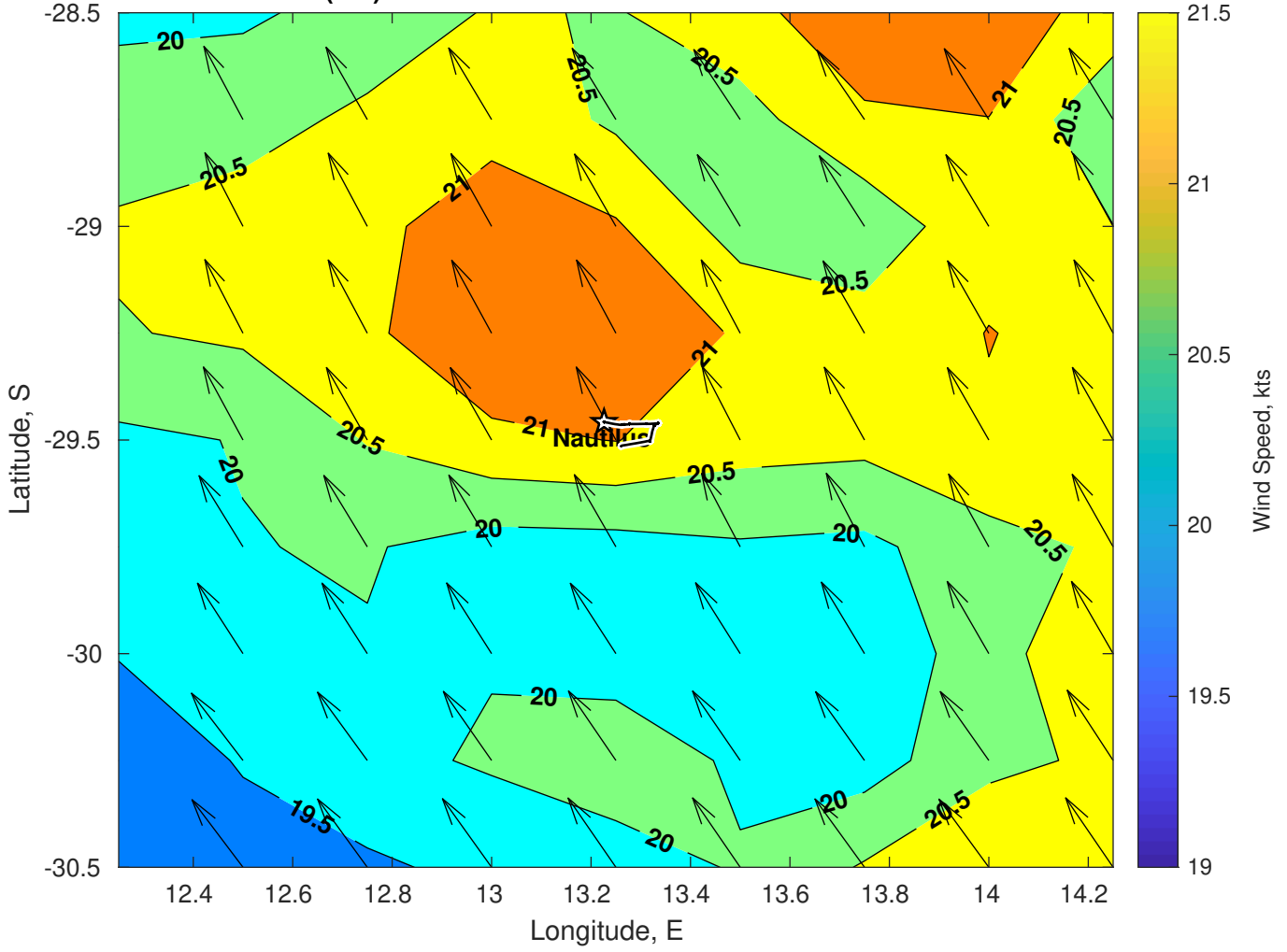
Winds (kts) for Nautilus at 13-Feb-2025 09:00:00
