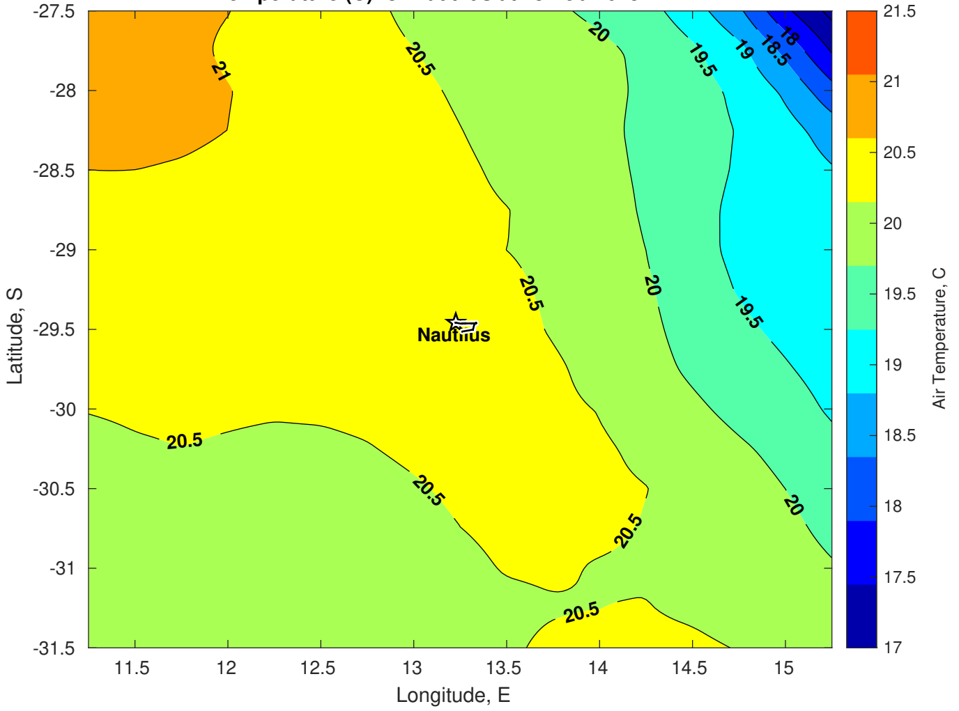
Air Temperature (C) for Nautilus at 13-Feb-2025
